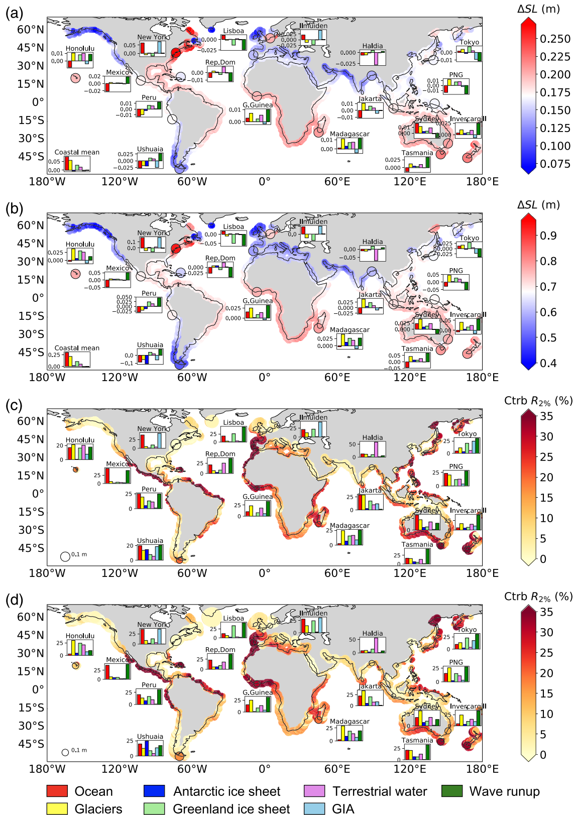
Figure 10. Spatial heterogeneity of the different contributions to projected coastal sea level changes, including runup. Same as Figure 7 but for wave runup changes instead of wave setup changes.
