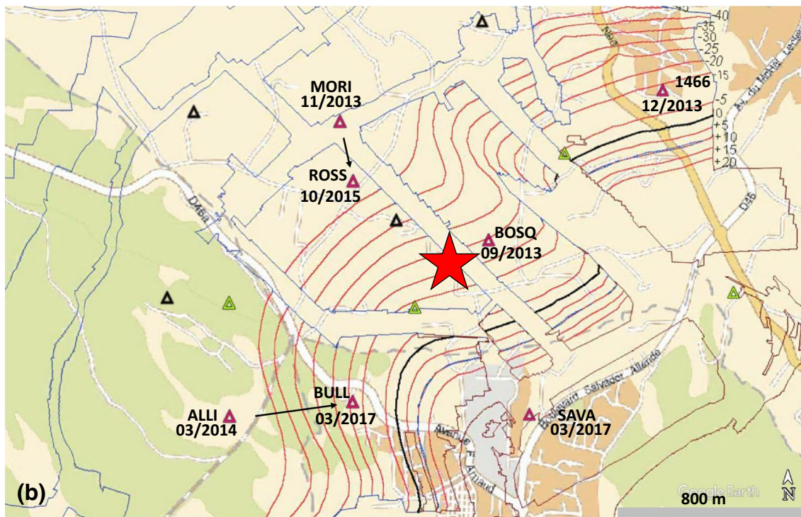
Fig. 4 Evolution of the temporary seismic BRGM network. a Five temporary BRGM stations (purple triangles) are superimposed on a map of the Gardanne coal basin. Ineris permanent network (green triangles). Main faults (bold black lines): DF Diote Fault, MF Meyreuil Fault, and JLF Jean-Louis Fault. Location of the seismic swarm in 2012 (red star). The pumping Gerard shaft (orange dot) and type of mine workings: room and pillars (vertical lines), long walls (dots),
