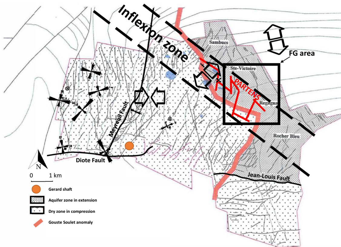
Fig. 2 Gardanne mine area with stress state (after Gaviglio 1987; Gaviglio et al. 1996, modified) separating the southwestern dry zone in compression and the northeastern aquifer zone in extension (after Chalumeau 2000, modified). Arrows represent magnitudes and orientations of the principal stresses determined for each site (Gaviglio et al. 2016). Large hollow arrows give the stress state (extension or
