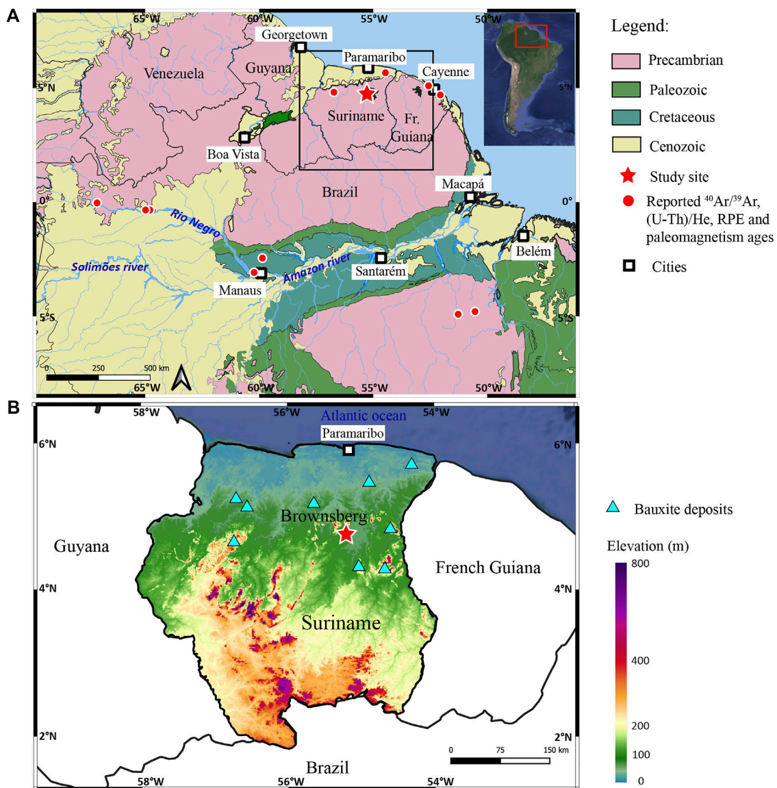
FIGURE 1 | (A) Simplified geological map of the Guiana shield (data from geosgb. cprm.gov.br) with location of dated laterites with ^{40}\text{Ar}/^{39}\text{Ar} , (U-Th)/He, EPR, or paleomagnetism on the Amazon craton (Vasconcelos et al., 1994; Théveniaut and Freyssinet, 2002; Balan et al., 2005; Allard et al., 2018; Heller et al., 2022) and (B) elevation map with known bauxite deposits in Suriname.
