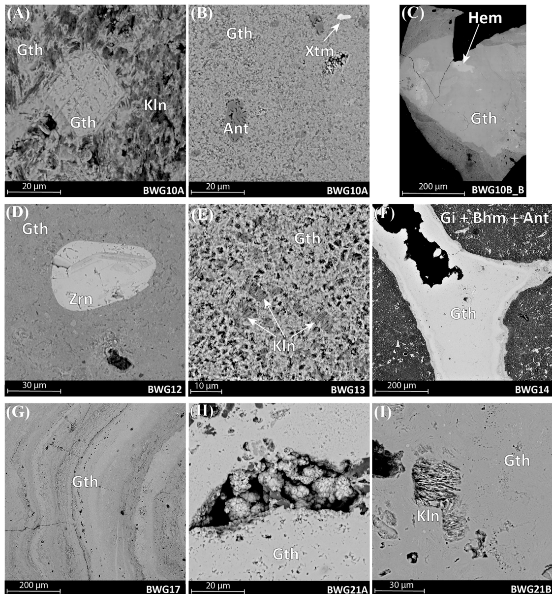
FIGURE 5 | Scanning electron microscopy images. (A) Detrital goethite (Gth) surrounded by intergrown kaolinite (Kln) booklets and checked secondary goethite. (B,D) Contaminant can be present in dated aliquots, for example, anatase (Ant), xenotime (Xtm), or zircon (Zrn). (C) Goethite is the main Fe-oxide found in the Brownsberg sample, but hematite (Hem) can be observed. (E,I) The massive duricrust from Leo Falls (BWG13) and the Mine (BWG21B) displays epigenetic replacement of kaolinite booklets by goethite. (F,G) Colloform goethite displaying various Al, Si, or Ti contents traduce long-term weathering under different environmental conditions. (F) The bauxite is mainly composed of gibbsite (Gbs) eventually accompanied by boehmite (Bhm) and anatase (Ant). (H) Polycrystalline texture of pure goethite in BWG21A.
