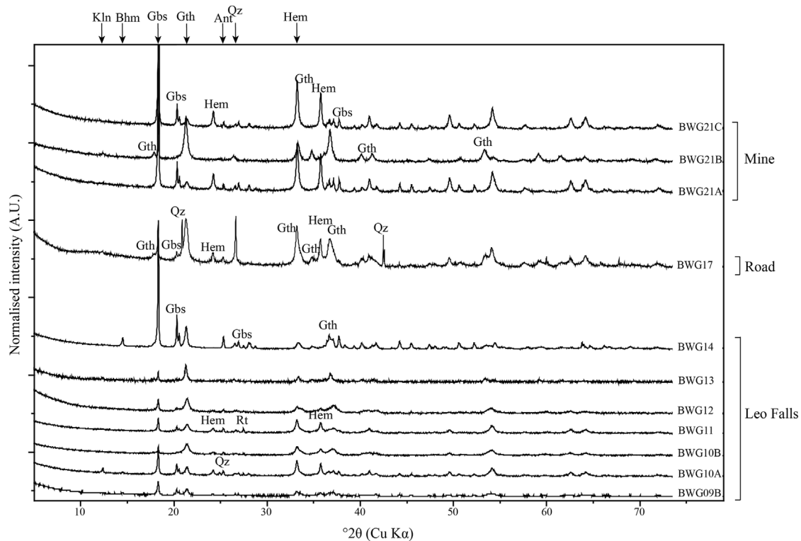
FIGURE 4 | XRD pattern of duricrust samples from each site. With Ant, anatase; Bhm, boehmite; Gbs, gibbsite; Gth, goethite; Hem, hematite; Kln, kaolinite; Qz, quartz; Rt, rutile.
