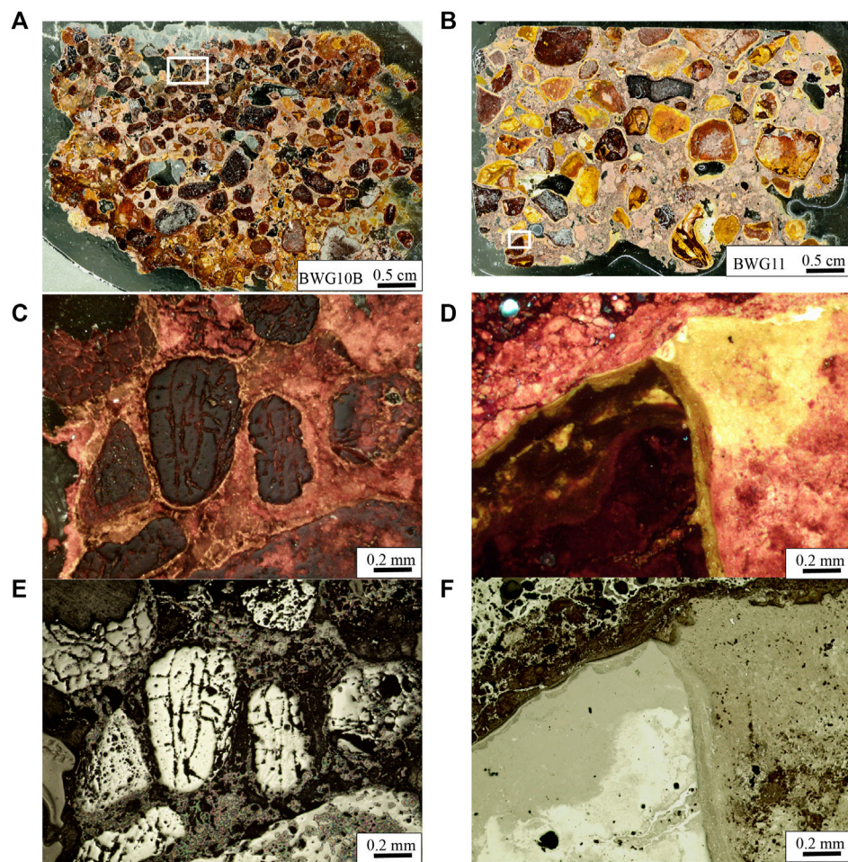
FIGURE 3 | Optical micro-photograph of thin sections of (A) BWG10B duricrust and (B) BWG11 duricrust, illustrating the Fe-oxide distribution. Magnified view of BWG10B (C) shows multiple Fe-oxide grains that look homogenous under reflected light (E) , while for BWG11 (D) , geochemical heterogeneities can be observed within a single isolated grain (F) .
