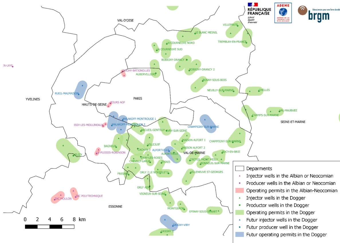
Figure 1: Localisation of the geothermal doublets tapping the Albian or Neocomian sands (pink) or the Dogger Limestones (green and blue) in Paris area
