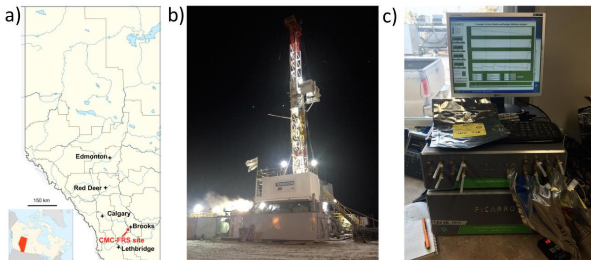
Fig. 1. a) Location of the Carbon Management Canada Research Institutes Inc. (CMC) Field Research Station (FRS) near Brooks (Alberta, Canada), b) drilling of well Countess 10-22-17-16W4 in Newell county near Brooks, and c) measurement of concentrations and \delta^{13}\text{C} values of methane in mud-gases at the site using cavity ring-down laser absorption spectroscopy.
