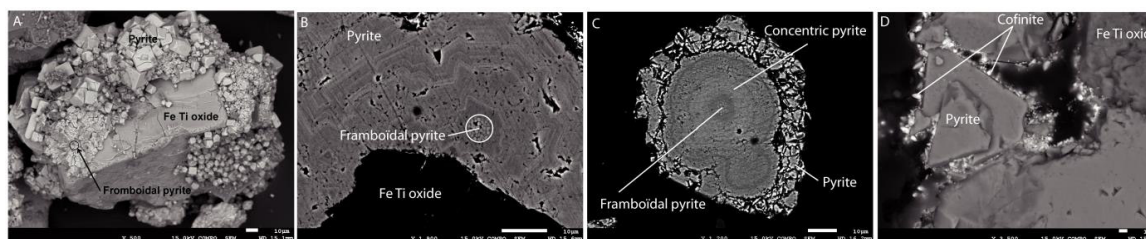
Fig. 1. Back-scattered electron images of pyrites with various morphology and there relations to Fe-Ti oxides and U-bearing minerals. (a) Fe-Ti oxide surrounded by different morphology of pyrite; (b) Polished section of the relation between the different generation of pyrite and Fe-Ti oxide, (c) example of the three main recognizable generation and there relations, (d) zoom on U-bearing mineral mineralized on the surface of pyrite and Fe-Ti-oxides.
