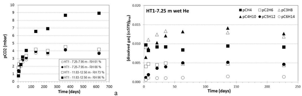
Fig. 1. Monitoring of gas partial pressures in HT core samples at Mont Terri (a) \text{CO}_{2(\text{g})} ; (b) concentrations of alkanes (given in ccSTP/g of pore water) in HT1-7.25 m core sample.
