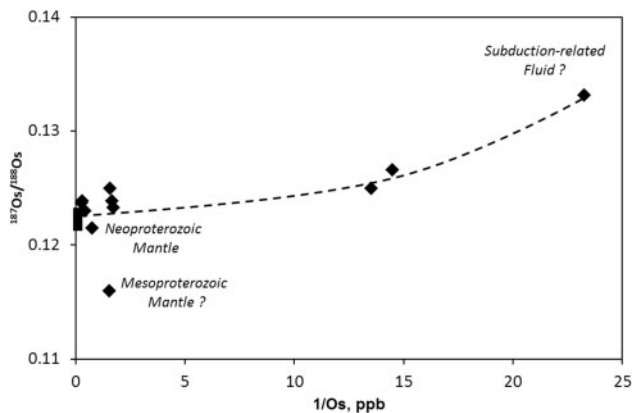
Fig. 11. ^{187}\text{Os}/^{188}\text{Os} vs 1/\text{Os} for dunites and pyroxenites from the Nizhny Tagil massif (filled diamonds). The trend of increasing Os isotopic composition with decreasing Os content (dotted line) can be ascribed to the admixture of subduction-related fluid. The least radiogenic ^{187}\text{Os}/^{188}\text{Os} value may indicate the ancient history of depletion. The in situ Os isotopic compositions of the PGM are also plotted (filled squares).
