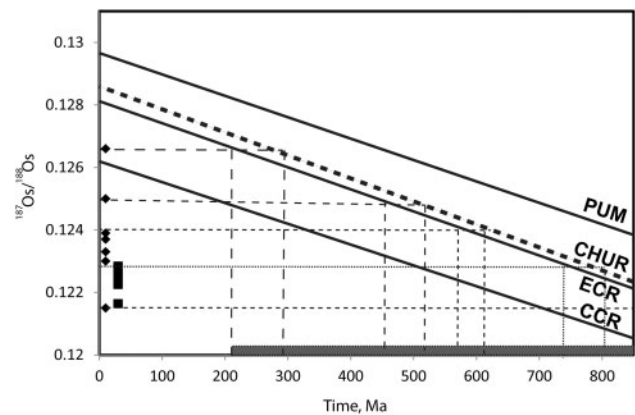
Fig. 12. Graphic representation of Os model ages for the Nizhny Tagil dunites and PGM estimated using different models for the Re–Os evolution of the convecting mantle [modified after Shi et al. (2007)]. Mantle evolution curves are defined as follows: CCR (Carbonaceous Chondrite reservoir) curve assumes that the Earth's mantle has an Os isotopic composition and \text{Re}/\text{Os} similar to that of carbonaceous chondrites ( ^{187}\text{Os}/^{188}\text{Os}_{\text{CC}} = 0.1262 \pm 0.0006 , ^{187}\text{Re}/^{188}\text{Os}_{\text{CC}} = 0.392 \pm 0.015 ; Walker et al. , 2002); ECR (Enstatite Chondrite Reservoir) curve is calculated using a present-day ^{187}\text{Os}/^{188}\text{Os} value of 0.1281 \pm 0.0004 and ^{187}\text{Re}/^{188}\text{Os} = 0.421 \pm 0.013 as measured in enstatite chondrites (Walker et al. , 2002); CHUR (Chondrite Uniform Reservoir) curve has initial ^{187}\text{Os}/^{188}\text{Os} of 0.09531, resulting in present-day ^{187}\text{Os}/^{188}\text{Os} = 0.12863 using ^{187}\text{Re}/^{188}\text{Os} = 0.423 (Chen et al. , 1998); PUM (Primitive Upper Mantle) curve has a present-day ^{187}\text{Os}/^{188}\text{Os} = 0.1296 \pm 0.0008 and ^{187}\text{Re}/^{188}\text{Os} = 0.42 . Grey band (X-axis) represent the time interval for Os model ages. Symbols as in Fig. 11.
