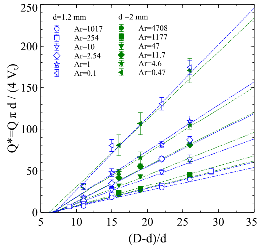
Figure 7: Dimensionless Q^* = Q\pi d/4V_t as a function of the dimensionless effective aperture (D-d)/d , for the whole set of simulations. The lines indicate linear fits.
