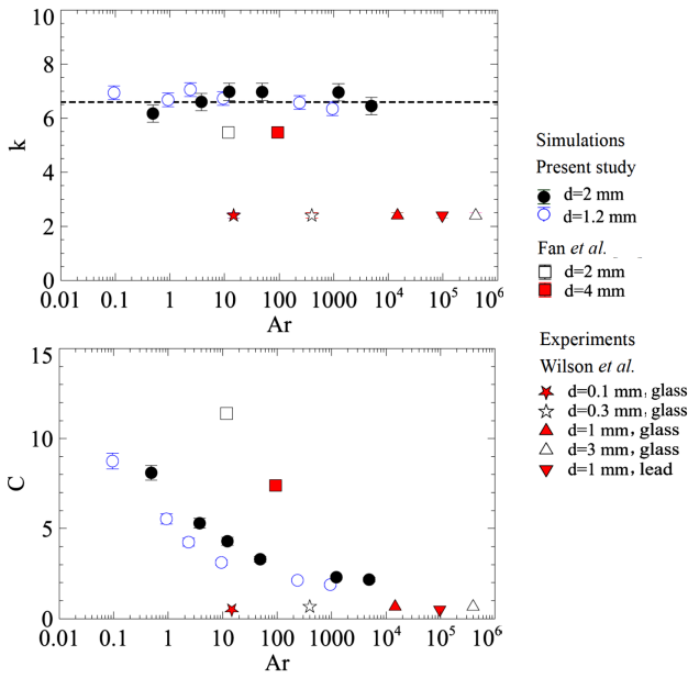
Figure 8: Parameters k and C of the 2D Beverloo law as a function of the Archimede numbers Ar , for the present simulations, a previous numerical study by Fan et al. [25], and experiments by Wilson et al. [24].
