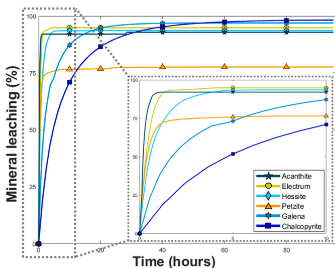
Fig. 7. Cumulative mineral leaching over 96 h of leaching simulation of acanthite, electrum, hessite, petzite, galena, and chalcopyrite for 322,842 particles.
