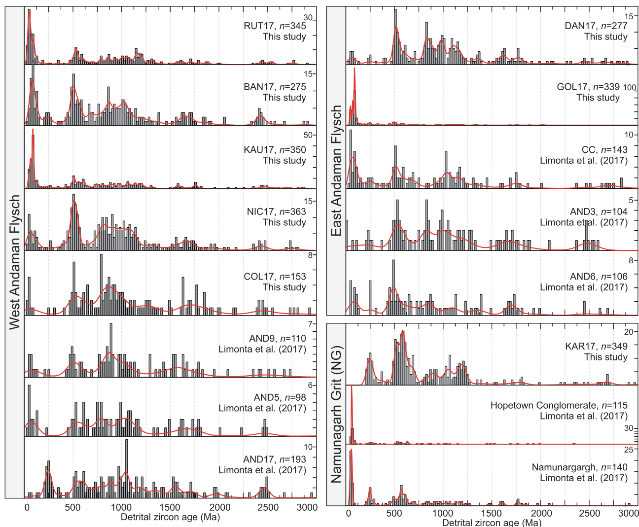
Fig. 11. Histograms and kernel density estimate diagrams for detrital zircon age distributions from the Namunargh Grit, East Andaman Flysch, and West Andaman Flysch (this study and Limonta et al., 2017). All ages are displayed in 20 Ma bins; number on y axis is the amount of zircon age per bin. Three NG samples from the Kalipur coast (2) and Mungleton (1) from Bandopadhyay and Carter (2017a) are not displayed because of low zircon number ( n < 80 ).
