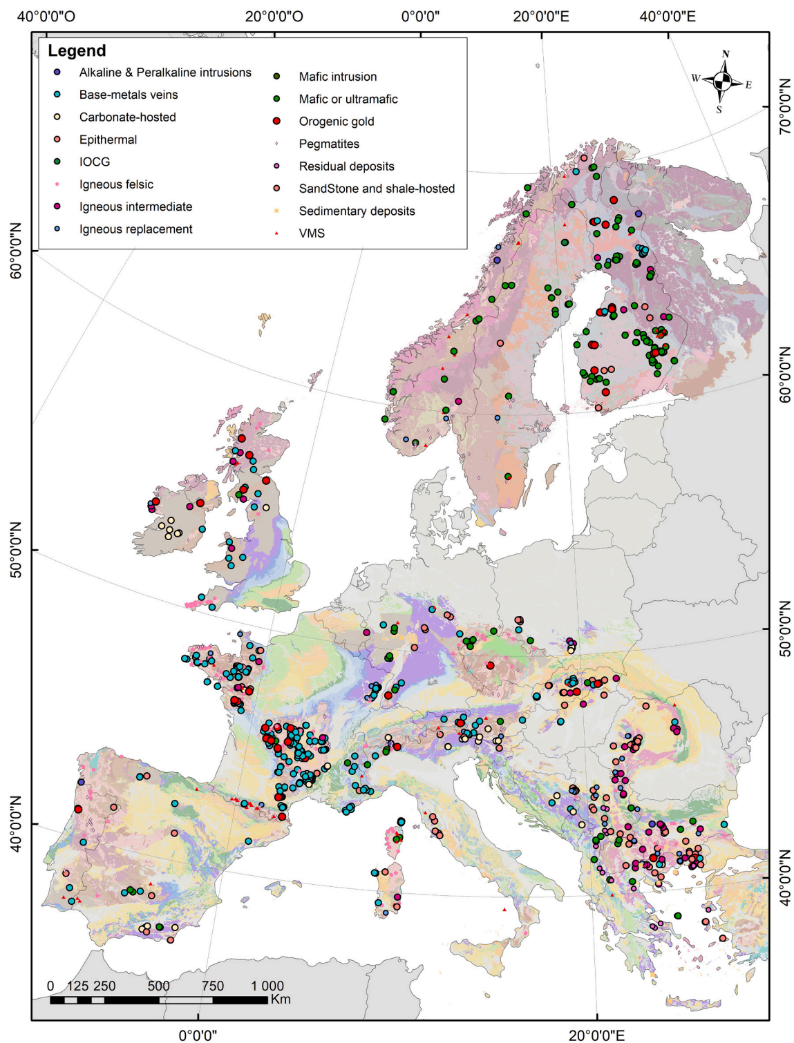
Fig. 2. Distribution of identified European Union occurrences ( n = 1400 ) showing identified ION4RAW targeted by-products classified according to their metallogenic family.
