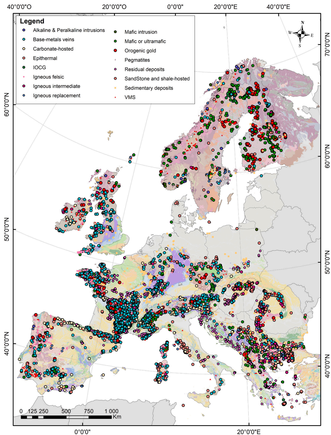
Fig. 1. Distribution of all European Union occurrences ( n = 8643 ) and deposits classified according to their metallogenetic family.
