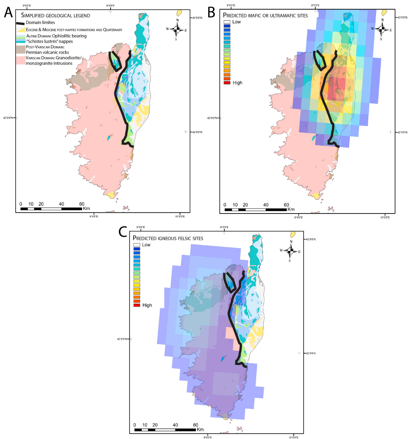
Fig. 12. Geological map of Corsica (A) and the respective predicted mafic/ultramafic (B) and the igneous felsic (C) metallogenic family maps.
