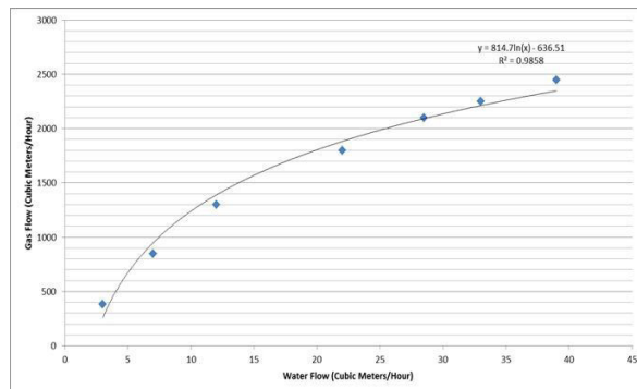
Figure 6 Fan et al.[11] data with natural log curve fit
