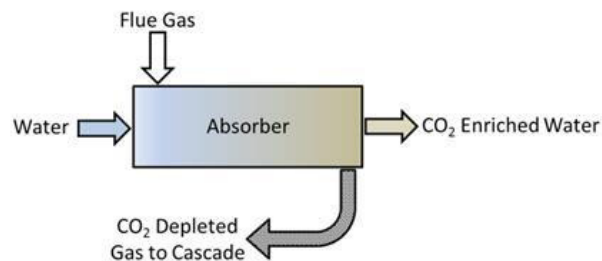
Figure 4 Simplified absorber diagram showing entries and exits
