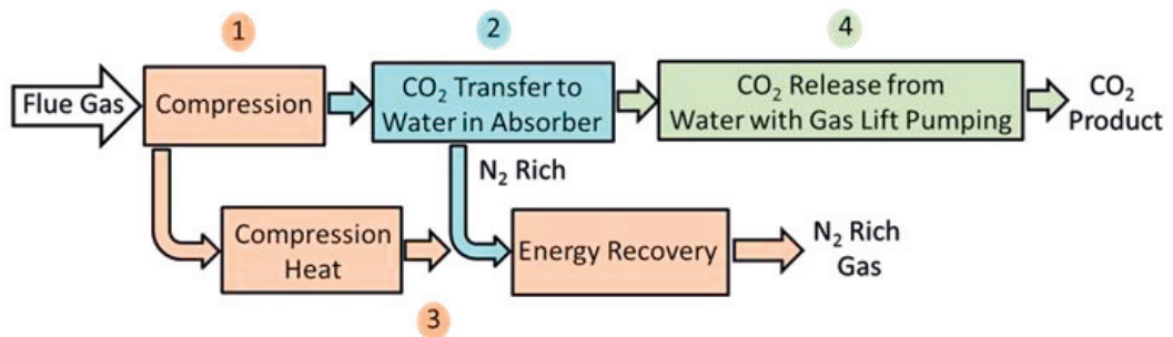
Figure 1 Generalized process steps for the Pi-CO 2 system
