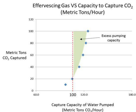
Figure 7 Effervescing gas versus capacity of the pumped water to capture CO 2
