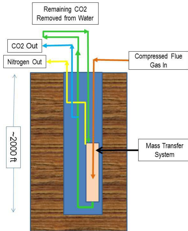
Figure 2 Simplified configuration of system
