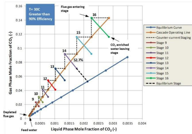
Figure 5 Modeled CO 2 absorption behavior in water using a multistage cascading absorber
