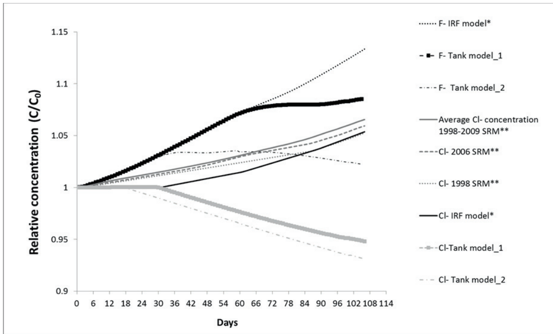
Fig. 4. Comparison between the relative aquifer solute concentration of chloride (Cl - ) simulated by the solute recycling model SRM ([1]**) and by the PHREEQC model for chloride (Cl - ) and fluoride (F - ) over one cycle of paddy field irrigation (dry season, [3]**) and one cycle of Tank infiltration (Tank model_1 = dry conditions 01/2006 to 04/2006; Tank model_2 = monsoon conditions 07/2012 to 10/2012).
