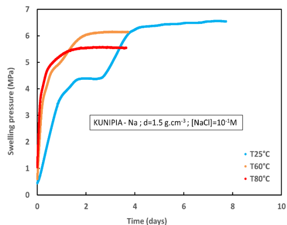
Figure 2: The swelling test results of a Kunipia-Na of density 1.5 g.cm -3 hydrated by a NaCl solution of concentration 10 -1 M at temperatures of 25, 60 and 80°C.
