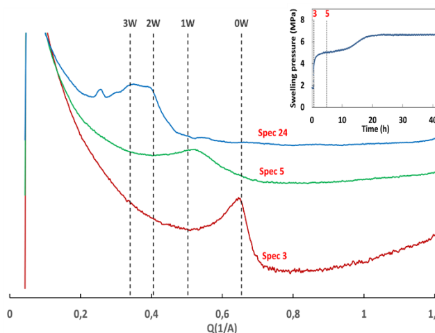
Figure 1: SAXS analysis performed on a Kunipia-Na of density 1.5 g.cm -3 hydrated by a NaCl solution of concentration 10 -1 M.
