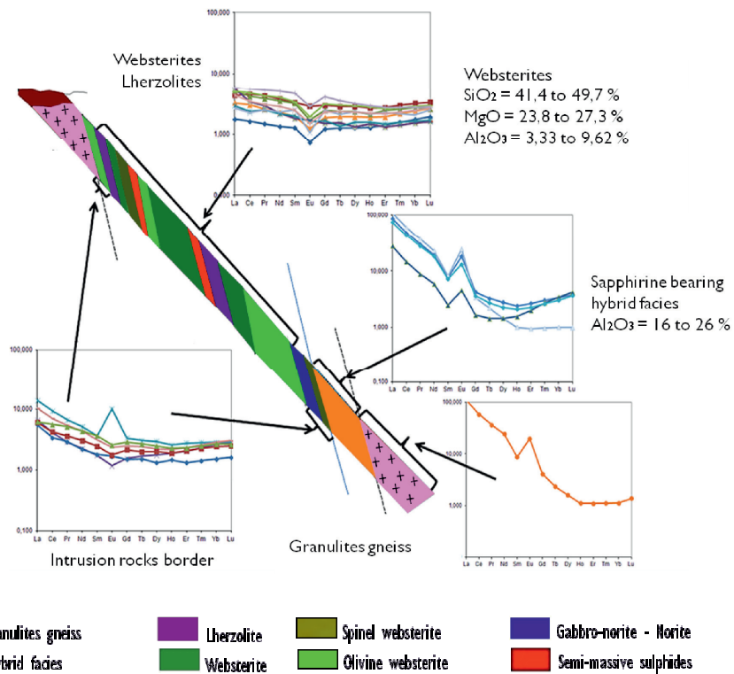
FIG. 6. – E1: SM24-661614 drilling log and proposed stratigraphic succession and associated rare earth geochemical signatures.
