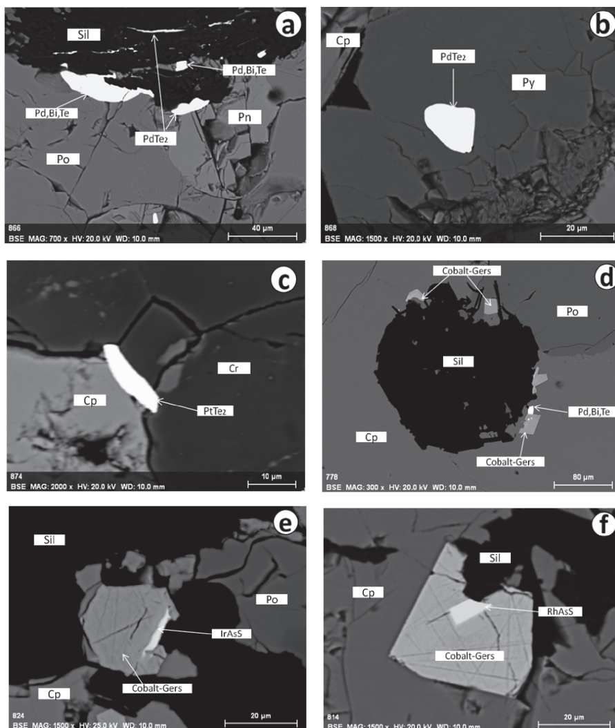
FIG. 9. – Microphotographs of various elements of the Platinum Group Minerals (PGM) at the Samapleu deposits obtained by scanning electron microscope. a: michenerite within Po on contact with silicate; merenskyite within Pn on contact with silicate and as dragged; b: merenskyite within pyrite; c: moncheite at the interface between chalcopyrite and chromite; d: (Rh, Pd) cobaltite-gersdorffite within (Cp, Po) sulfides; e: irarsite exsolution within cobaltite-gersdorffite; f: hollingworthite exsolution within cobaltite-gersdorffite. Sil = Silicate; Cr = chromite; Po = pyrrhotite; Pn = pentlandite; Cp = chalcopyrite; Cobalto-Gers = cobaltite-gersdorffite; RhAsS = hollingworthite; IrAsS = irarsite; PtTe2 = moncheite; PdTe = merenskyite; Pd,Bi,Te = michenerite.
