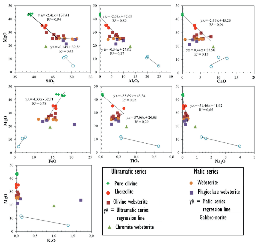
FIG. 7. – Major element diagrams (SiO 2 , Al 2 O 3 , CaO, Na 2 O, FeO, TiO 2 and K 2 O) with MgO of Samapleu sequence cumulates. R 2 = distribution coefficient.
