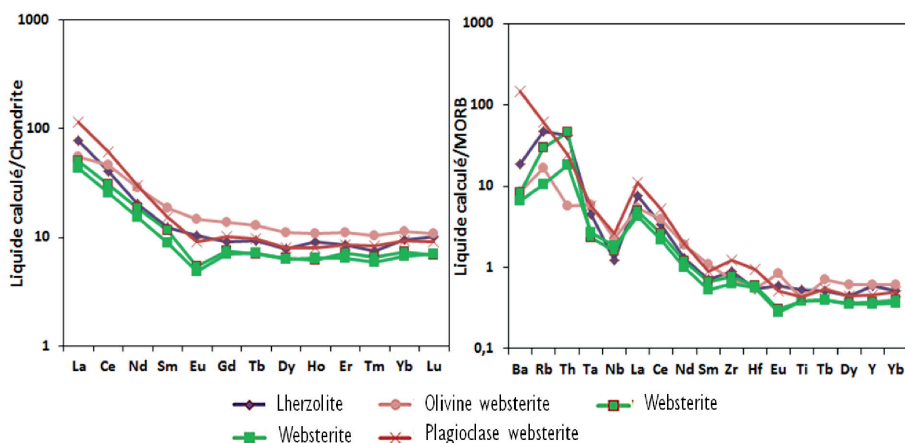
FIG. 12. – Rare earth and trace elements signatures of E1 lithological units at equilibrium [Bédard, 1994].
