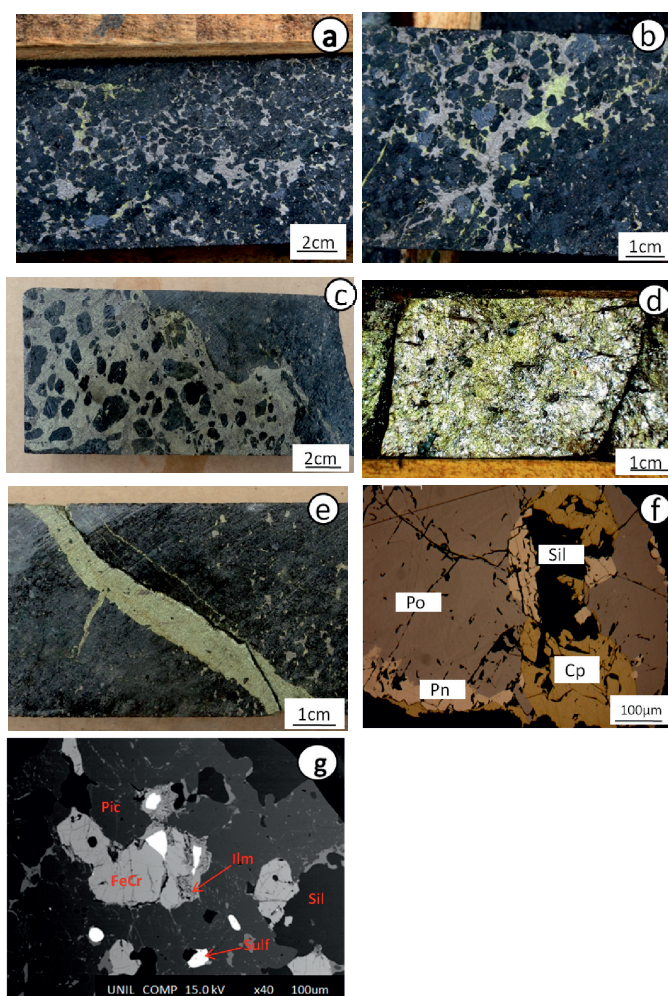
FIG. 8. – Photography of various sulfide textures and oxides observed at the Samapleu deposits. A: matrix texture; b: net texture; c: breccia texture; d: massive sulfide; e: late chalcopyrite veins; f: photomicrographs in reflected light of pyrrhotite (Po), pentlandite (Pn), chalcopyrite (Cp), Sil (silicates); g: chromites (UNIL microprobe). Pic = picotite; FeCr = ferrochromite; Ilm = ilménite; Sulf = sulfure.
