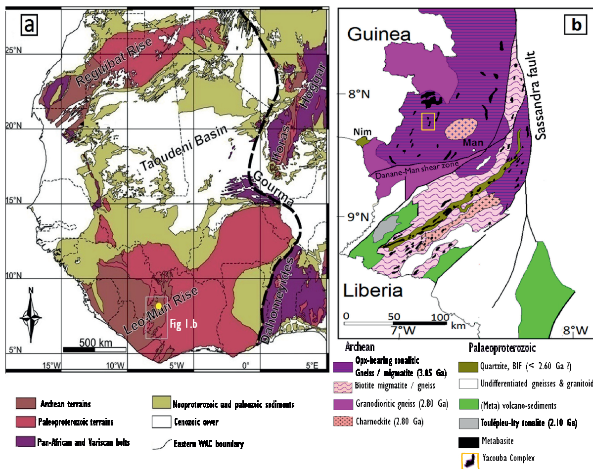
FIG. 1. – Schematic geological map. A: West African shield [Berger et al. , 2013]; b: Man craton in western Côte d'Ivoire [Pitra et al. , 2010]. Figure 1b window shows the Sipilou-Biankouma area and the Yacouba layered complex as it is currently known.
