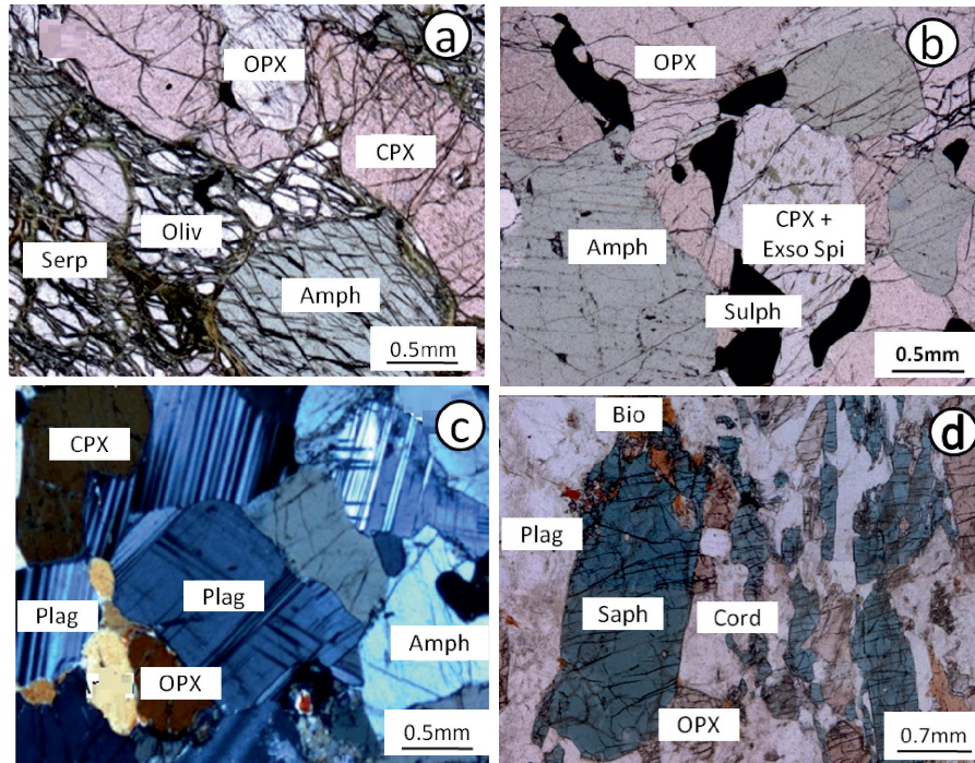
FIG. 5. – Photomicrographs of various members of the Samapleu intrusion. A: partially serpentinized lherzolite; b: pyroxenite; c: gabbro-norite; d: hybrid zone with sapphirine. Bio = biotite; Plag = plagioclase; Saph = sapphirine ; Serp = serpentine; Amph = amphibole ; Oliv = olivine ; Cord = cordierite ; CPX = clinopyroxene ; OPX = orthopyroxène; Sulph = sulfide; Exso Spin = exsolution spinel
