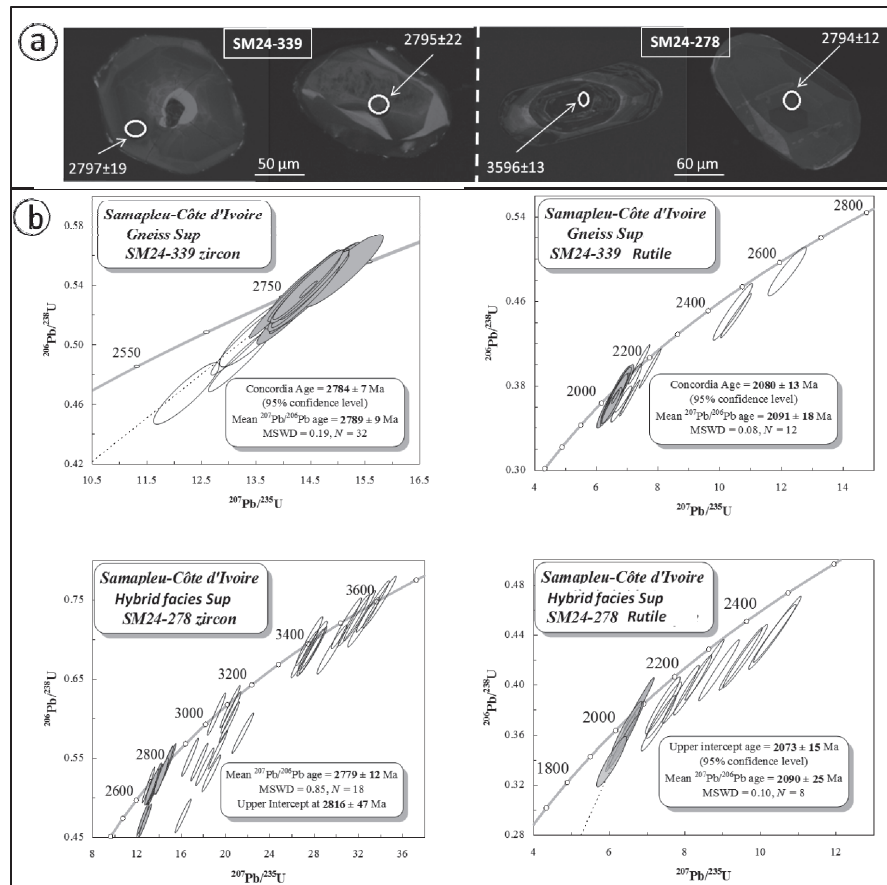
FIG. 10. – Radiochronologic analysis performed in the LMV in Clermont Ferrand University on gneisses and the hybride zone of the E1 zone at the contact between the intrusion and the surrounding rocks. A – Pictures of selected zircon grains; the circles represent the position of laser spots used for age determination, and the associated values are the resulting ^{207}\text{Pb}/^{206}\text{Pb} age (in Ma). B – Concordia plots ( ^{206}\text{Pb}/^{238}\text{U} vs. ^{207}\text{Pb}/^{235}\text{U} ) performed from zircons and rutile.
