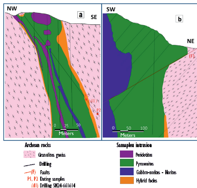
FIG. 4. – Cross-section showing Samapleu mafic-ultramafic sequences from borehole data. a: Line AA' Samapleu Extension 1 (fig. 3a); b: Line BB' Samapleu Main (fig. 3a).
