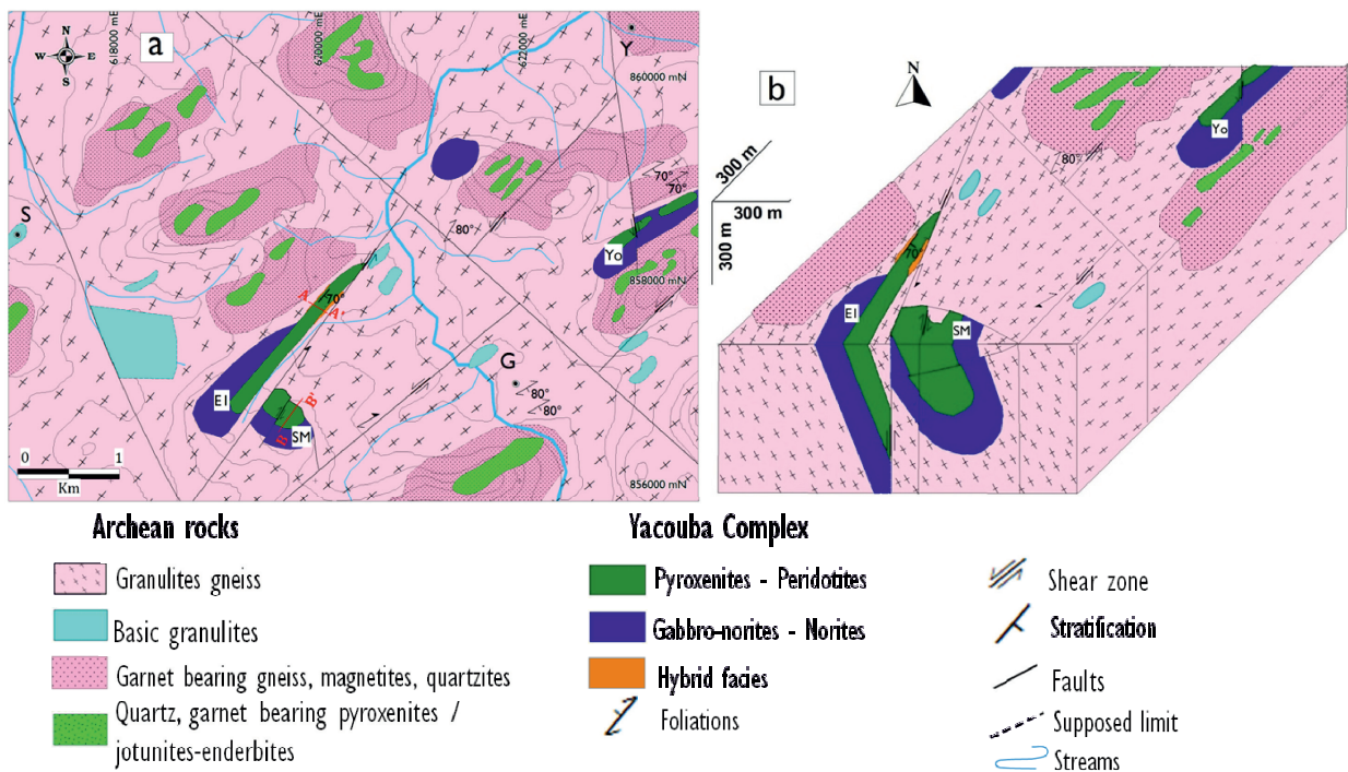
FIG. 3. – The Yacouba layered complex members including: Samapleu mafic-ultramafic sequences in the Samapleu-Yorodougou area, together with gneissic granulite and quartzite country rock. a: schematic geological map; b: block diagram. Samapleu Extension 1 = E1; Samapleu Main = SM; Yorodougou occurrence = Yo; Samapleu = S; Gangbapleu = G; Yorodougou = Y.
