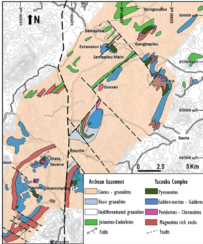
FIG. 2. – The Yacouba layered complex members including: Samapleu mafic and ultramafic facies near Yorodougou - Samapleu - Gangbapleu and Bounta villages in the Biankouma region. Samapleu Extension 1 = E1;
