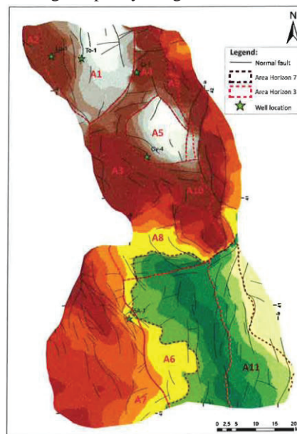
Fig.3. Depth representation of the Torres Vedras Formation in the Porto Basin, including fractures (Carneiro et al, 2011)
