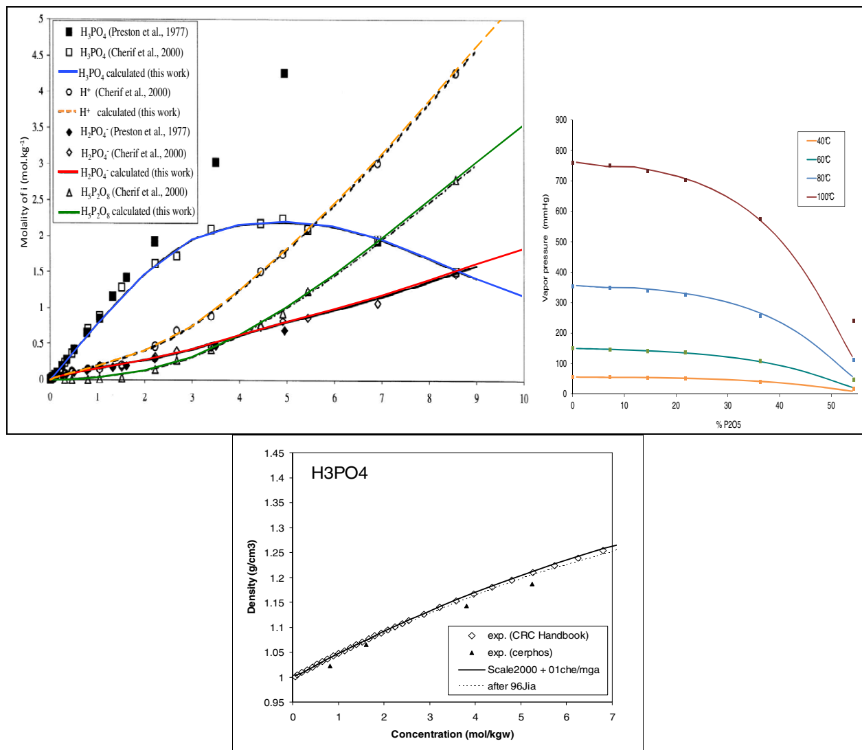
Figure 5 - Typical calculations for phosphate industry obtained with SCALE2000 (V5.0): detailed phosphoric acid speciation (H 3 PO 4 , H 2 PO 4 - , H 3 P 2 O 8 ) on the upper left figure, practice abacuses at several temperatures using the « Abacuses Menu » on the upper right figure and density of concentrated aqueous phosphate solutions on the lower figure.
