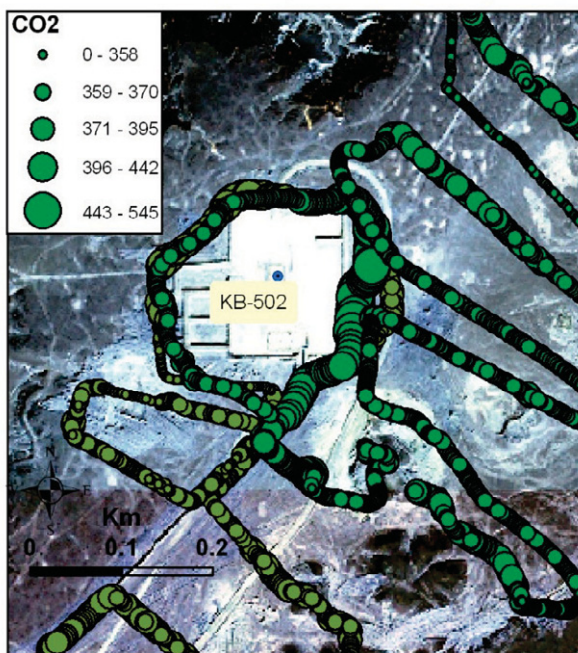
Figure 2. Data for near ground atmospheric \text{CO}_2 (concentrations in ppm) from mobile open path laser measurements around KB-502. Note higher values to the east and NW of the well due to vehicle exhaust affecting measurements with the laser probe
