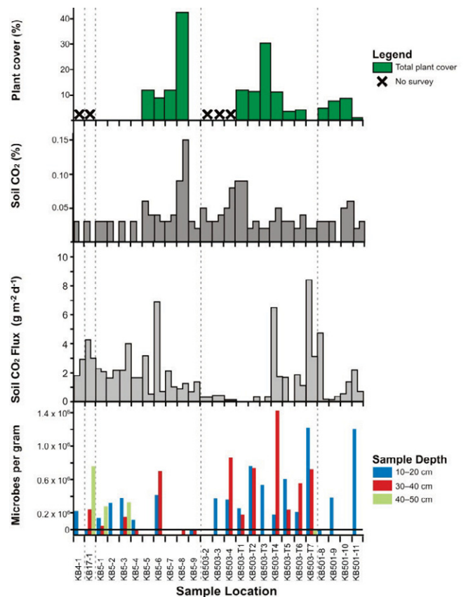
Figure 4. Comparison of microbial counts, soil \text{CO}_2 concentration and plant coverage datasets.
