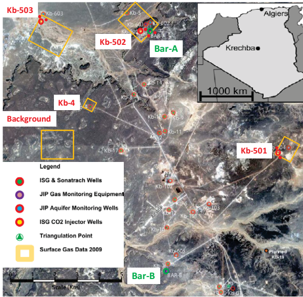
Figure 1. Location map of Krechba field on Quickbird satellite image with main study areas. Bar-A and Bar-B are Barasol locations. Solid red dots are passive sensor locations. Inset map shows location of Krechba in Algeria
