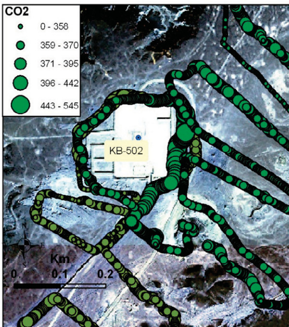
Figure 2. Data for near ground atmospheric CO 2 (concentrations in ppm) from mobile open path laser measurements around KB-502. Note higher values to the east and NW of the well due to vehicle exhaust affecting measurements with the laser probe
