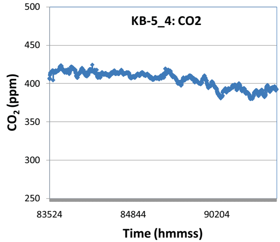
Figure 3. Static measurement of near ground atmospheric CO 2 SE of KB-5 in area of apparently higher CO 2 . Note decline with time
