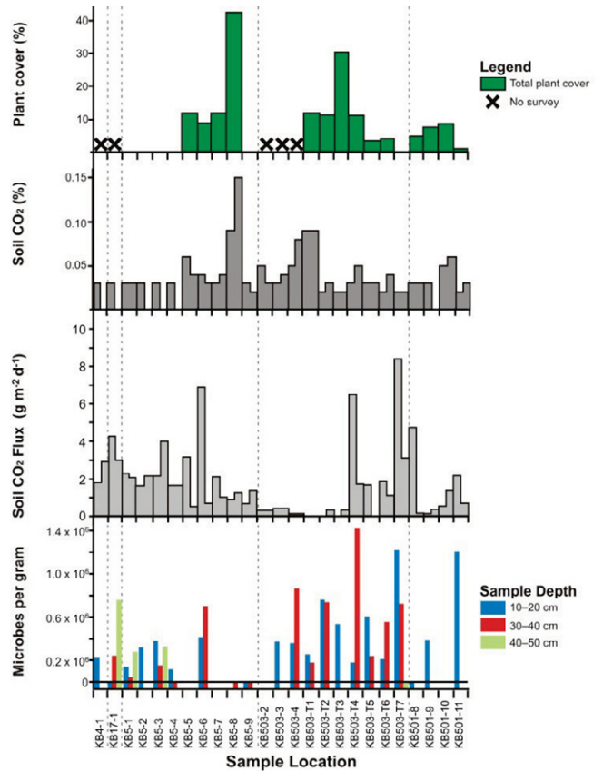
Figure 4. Comparison of microbial counts, soil CO 2 concentration and plant coverage datasets.
