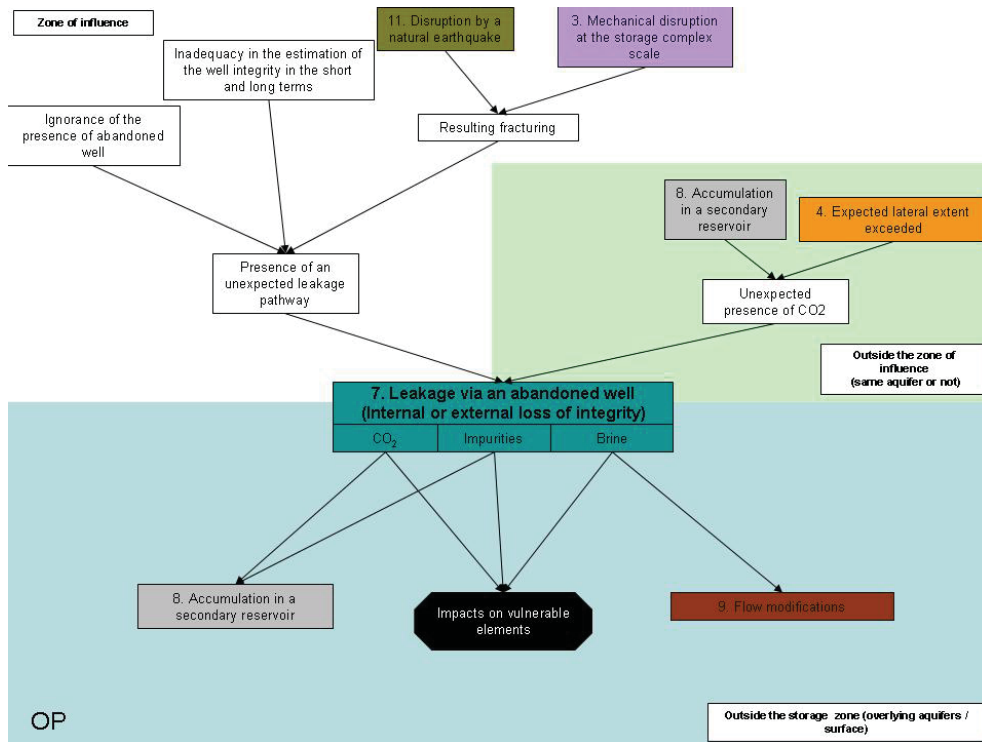
Figure 2: Operational phase diagram for event n°7: "Leakage via an abandoned well"
