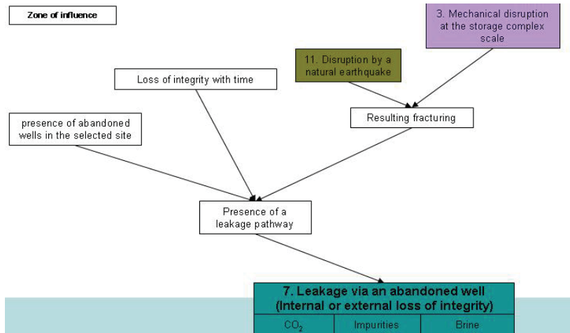
Figure 1: Planning phase diagram for event n°7: "Leakage via an abandoned well". Only the upper part of the diagram is shown, as consequences are similar to the operational phase diagram.
