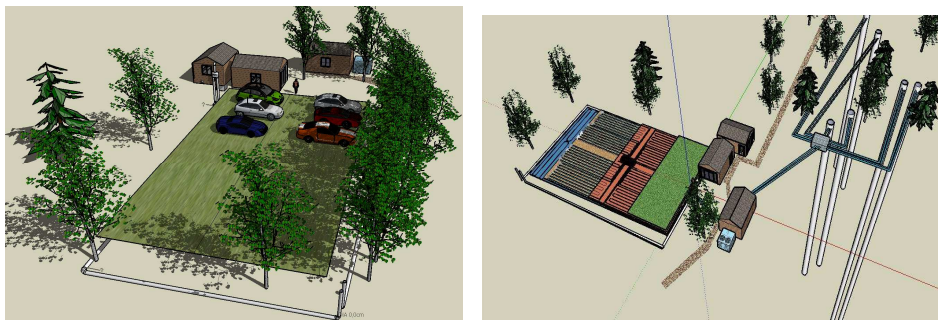
Figure 1. Artist views of the platform, made of horizontal & vertical heat exchangers equipped with optical fiber cables
