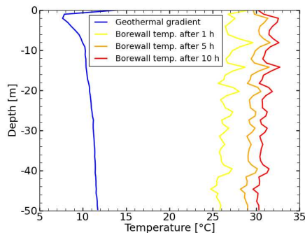
Figure 3. Natural geothermal gradient and temperature curves along the borewall after heat injection at 35°C during 1, 5 and 10 hours
