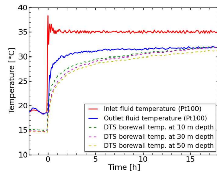
Figure 4. Underground temperature sensing (PT100 & DTS) while hot fluid (35°C) is injected in the GHE
