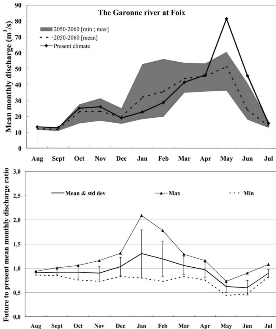
Figure 8. (top) Mean monthly discharges simulated at the Foix hydrometric station for the present decade (1985–1995) and the future decade (2050–2060, mean value and envelope curve containing the mean monthly discharge values simulated in the seven scenarios and limited by the extreme values for each month). (bottom) Ratios of the mean monthly discharges simulated under the climate scenarios to the mean monthly discharges simulated under the present climate (mean monthly value along with the standard deviation range and extreme values for each month).
