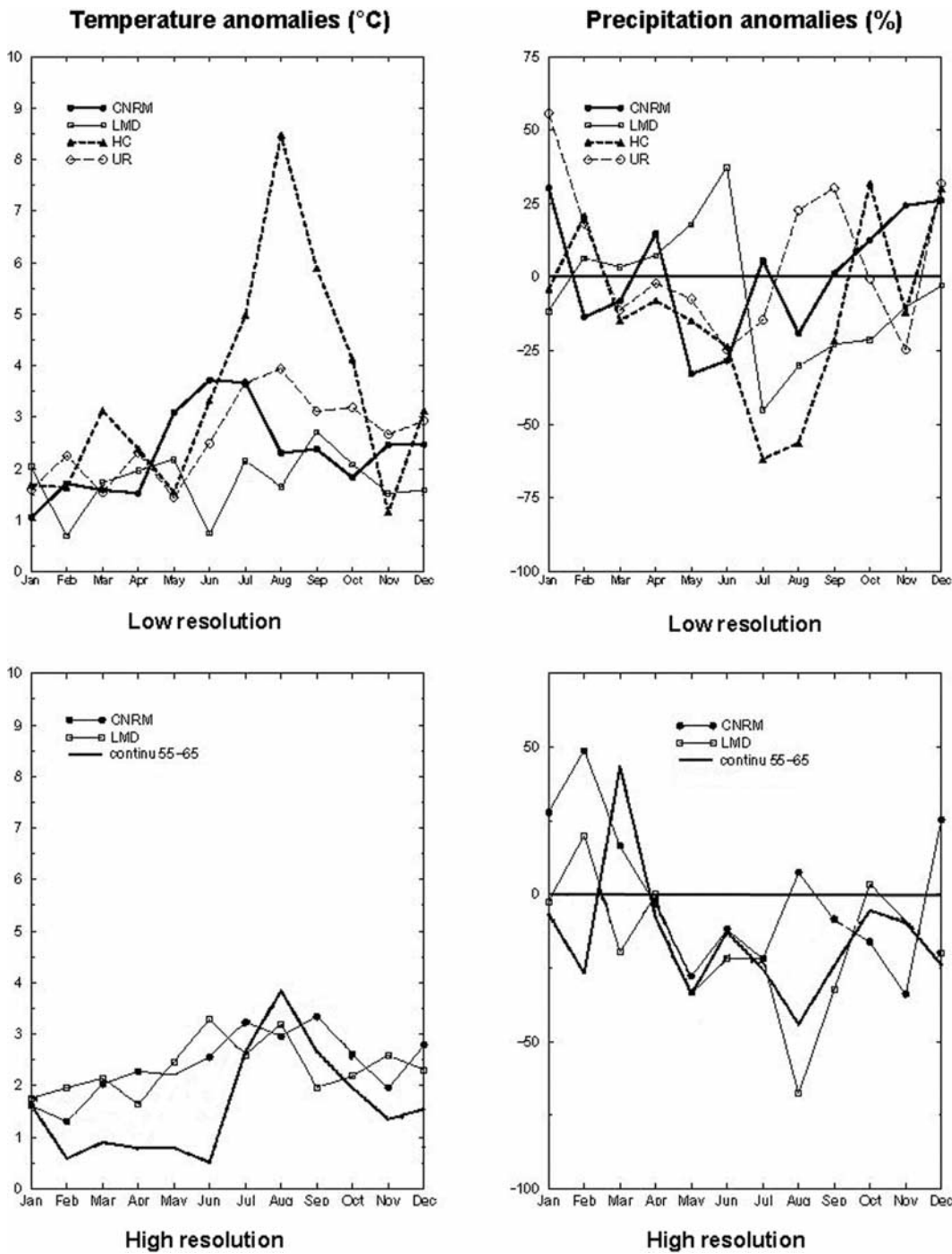
Figure 7. Monthly temperature and precipitation anomalies calculated from the seven GCM outputs for the present (1985–1995) and the modified climate (2050–2060) averaged over the region studied (modified from Lehenaff [2002]). The Action Recherche Petite Echelle et Grande Echelle (ARPEGE) continuous scenario anomalies are available for the 2055–2065 decade.
