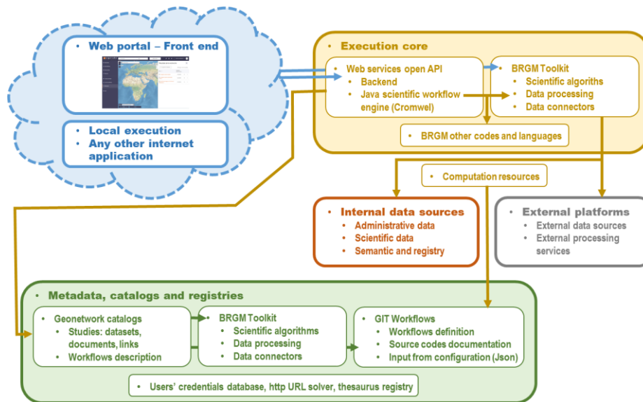
Figure 1: Vigirisks architecture
