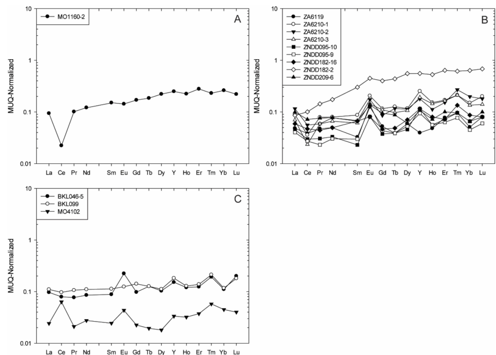
Figure 6. MUQ-normalized REE + Y patterns for BIF samples in different parts of the Chaillu Block: (A) Mayoko, (B) Zanaga, and (C) Bikélélé.
