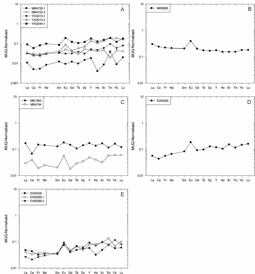
Figure 5. MUQ-normalized REE + Y patterns for BIF samples in different parts of the Kelle-Mbomo Block: (A) Youkou, (B) Kékélé, (C) Ngoyboma, (D) Obélé, and (E) Odia.
