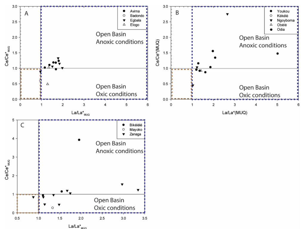
Figure 9. Binary plots of Ce/Ce^*_{MUQ} versus La/La^*_{MUQ} for the Ivindo (A), Kelle-Mbomo (B) and Chaillu (C) blocks. The blue dashed box is the open basin environment, whereas the brown dashed box represents the closed basin in which Fe-oxyhydroxide drives REE-Y scavenging.
