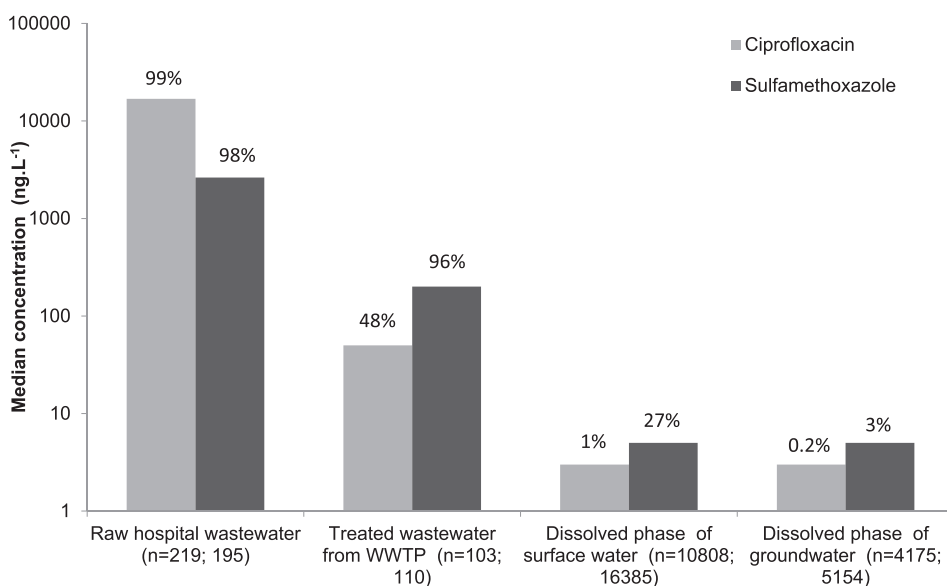
Fig. 5. Median concentrations of ciprofloxacin and sulfamethoxazole and proportion of samples above the limit of detection along the contamination continuum. The numbers of samples for ciprofloxacin and sulfamethoxazole are indicated in brackets, in this order). See Supplemental Table 1 for details. We substituted results below the analytical limit with half of the detection limit value. The labels on top of the bars give the proportion of samples above the limits of detection (LOD; 6 ng.L -1 for ciprofloxacin and 10 ng.L -1 for sulfamethoxazole (Patrolecco et al., 2018)).
