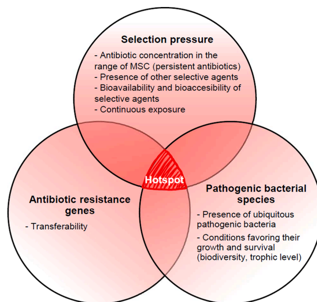
Fig. 3. Environmental conditions favorable to the transfer of antibiotic resistance genes to pathogenic bacterial species. MSC, minimal selective concentration.
