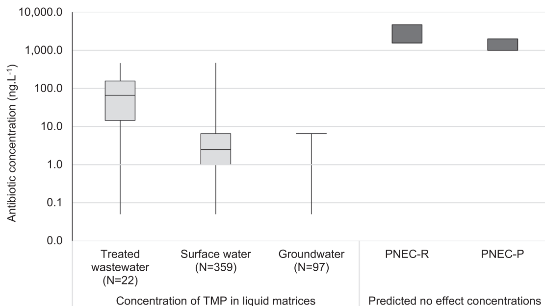
Fig. 7. Antibiotic concentrations in the dissolved phase of various liquid environmental matrices (antibiotic alone in light gray; sum of all antibiotic residues from the same class in dashed grey) and the predicted no effect concentration for resistance (PNEC-R) and for persistence (PNEC-P) (dark gray) for ciprofloxacin (panel A), trimethoprim (panel B), macrolides (panel C) and tetracycline (panel D). FQ, fluoroquinolones; TMP, trimethoprim; ML, macrolides; TC, tetracyclines; N, number of samples; PNEC values were taken from (Murray et al., 2021). The PNEC values were those of ciprofloxacin (panel A; PNEC-R, 50–780 \text{ng.L}^{-1} ; PNEC-P, 10 \text{ng.L}^{-1} ), trimethoprim (panel B; PNEC-R, 1,560–3,130 \text{ng.L}^{-1} ; PNEC-P, 1,000 \text{ng.L}^{-1} ), azithromycin, clarithromycin (panel C; PNEC-R, 50,000–12,500,000 \text{ng.L}^{-1} ; no PNEC-P yet defined), tetracycline (panel D; no PNEC-R yet defined; PNEC-P: 10 \text{ng.L}^{-1} ).
