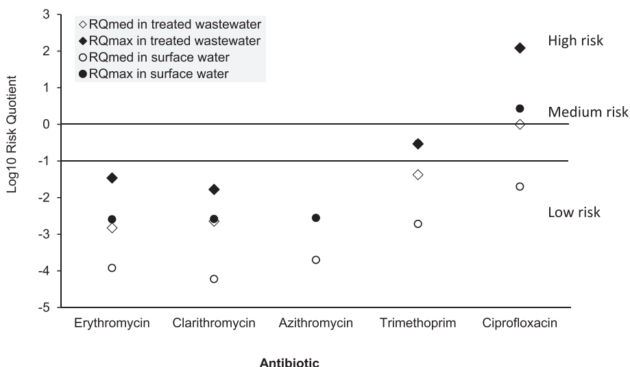
Fig. 8. Risk quotients (RQs) for aquatic environments (treated wastewater and surface water) in France. RQ max (RQ maximum) and RQ med (RQ median) were based on maximum and median measured environmental concentrations (MECs) divided by the PNEC-R determined experimentally with the SELECT method (Murray et al., 2020). MECs were extracted from Supplemental Table 1. RQs were represented on a logarithmic scale. High, medium, and low risks were defined by Log 10 RQ values > 0, -1 to 0, and < -1, respectively. We kept for analysis antibiotics whose MEC was assessed > 10 times and which were above the detection limit in > 10 % of the cases.
