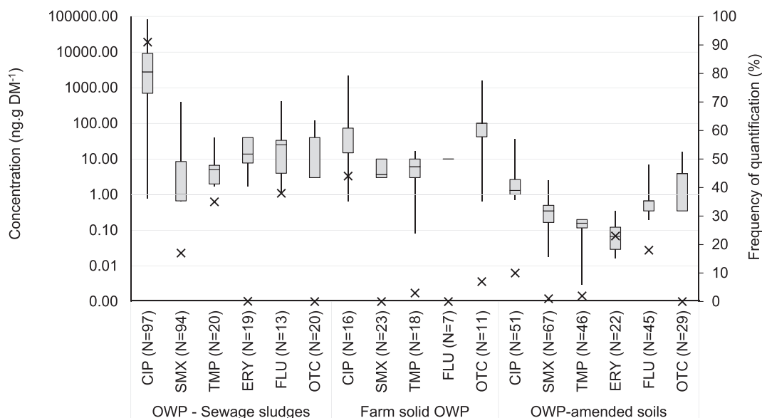
Fig. 6. Concentrations of six antibiotics from different pharmacological classes measured in OWPs (sewage sludges and solid farm products) and in OWP-amended soils in France. The antibiotics considered are those for which the largest amount of data was available in their pharmacological class, for all the considered matrices. Concentrations are presented as box plots (min, P25, median, P75, and max; left y-axis) and quantification frequencies as crosses (right y-axis). Results below the analytical limit were substituted by half of the detection limit value. All the dosage of ERY in solid farm product ( n = 4 ) were below the LOD and not represented. CIP, ciprofloxacin (fluoroquinolone); SMX, sulfamethoxazole (sulfonamide); TMP, trimethoprim; ERY, erythromycin (macrolide); FLU, flumequine (quinolone); OTC, oxytetracycline (tetracycline); OWPs, Organic Waste Products; N, number of samples; DM, dry matter. For amended soils: (Bourdat-Deschamps et al., 2017; Dinh et al., 2017b; Nazaret, 2020a,b; Salvia et al., 2015; Salvia et al., 2012; Tamtam et al., 2011a); for farm solid OWP: (Algros and Jourdain, 2007; Bourdat-Deschamps et al., 2017; Moraru et al., 2012; Nazaret, 2020a,b; Pourcher et al., 2014; Simonet and Gardeur-Algros, 2012); for sewage sludges: (Algros and Jourdain, 2007; Bourdat-Deschamps et al., 2017; Simonet and Gardeur-Algros, 2012; Tamtam et al., 2009).
