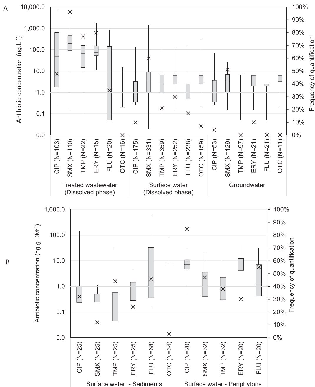
Fig. 4. Concentration of antibiotics from different pharmacological classes in the dissolved phases of treated wastewater, surface and groundwater (A) and in aquatic sediments and periphytons (B) in France. Box plots indicate min, P25, median, P75 and max of antibiotic concentrations (left y-axis). The crosses indicate the frequencies of quantification (right y-axis). The antibiotics considered are those for which sufficient data were available for all the matrices (we chose an arbitrary cutoff of 10 data points). We substituted results below the analytical limit with half of the detection limit value. CIP, ciprofloxacin (fluoroquinolone); SMX, sulfamethoxazole (sulfonamide); TMP, trimethoprim; ERY, erythromycin (macrolide); FLU, flumequine (quinolone); OTC, oxytetracycline (tetracycline); N, number of samples; DM, dry matter (Aubertheau-Laurent, 2013; Azimi et al., 2018; Camilleri et al., 2015; Capdeville, 2011; Chonova et al., 2016; Chonova et al., 2018; Coetsier et al., 2009; Dinh et al., 2017a; Feitosa-Felizzola and Chiron, 2009; Garcia-Armisen et al., 2013; Guibal et al., 2018; Joigneaux, 2011; Mailler et al., 2015; Tamtam et al., 2008; Wiest et al., 2018).
