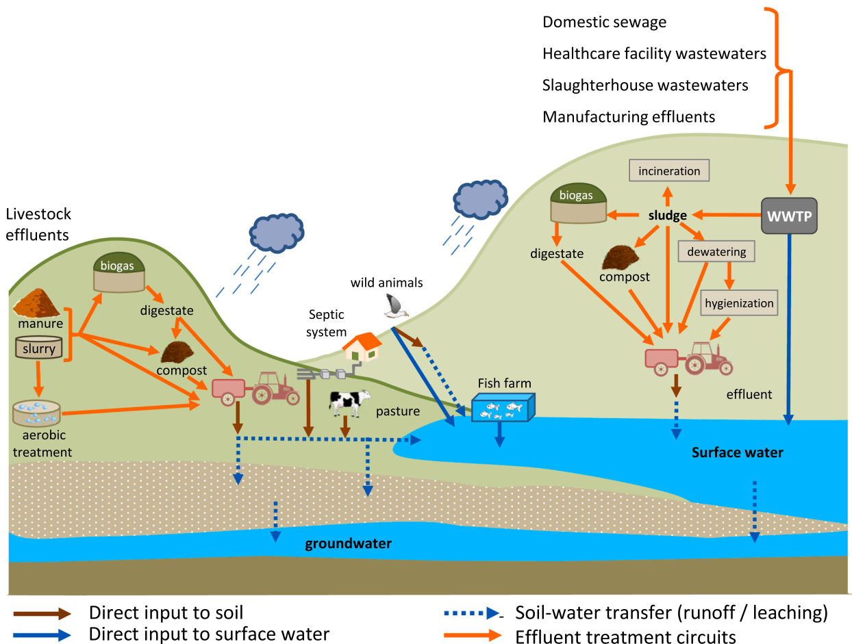
Fig. 2. Main sources and contamination routes of soil and water by antibiotic-resistant bacteria and antibiotic residues. WWTP, wastewater treatment plant.
