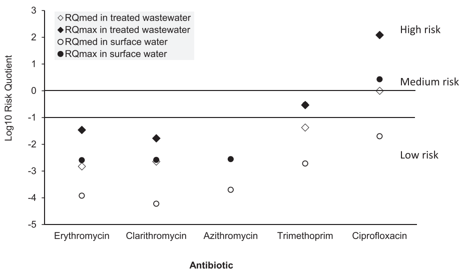
Fig. 8. Risk quotients (RQs) for aquatic environments (treated wastewater and surface water) in France. RQ_{max} (RQ maximum) and RQ_{med} (RQ median) were based on maximum and median measured environmental concentrations (MECs) divided by the PNEC-R determined experimentally with the SELECT method (Murray et al., 2020). MECs were extracted from Supplemental Table 1. RQs were represented on a logarithmic scale. High, medium, and low risks were defined by \text{Log}_{10} RQ values > 0 , -1 to 0 , and < -1 , respectively. We kept for analysis antibiotics whose MEC was assessed > 10 times and which were above the detection limit in > 10\% of the cases.
