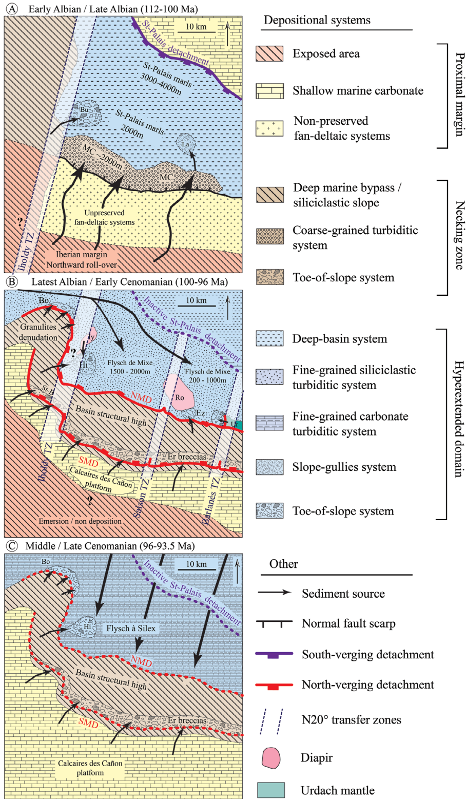
Fig. 11. Palinspastic restorations of the Mauléon hyperextended rift basin showing the main depositional systems, active faults and sedimentary fluxes from the Albian to the Late Cenomanian. (A) Early to Late Albian; (B) latest Albian to Early Cenomanian; (C) Middle to Late Cenomanian. Bu: Bustince Formation; MC: Mendibelza Formation; La: Lanne Member; SMD: South Mauléon Detachment; NMD: North Mauléon Detachment; Er: Errozaté Formation; St-B: Saint-Étienne-de-Baïgorry Formation; Bo: Bonloc Formation; Hi: Hiruraitzeta Formation; Ez: Erretzu Member; Ur: Urdach Member; Iy: Iholdy diapir; Ro: Roquiague diapir.
