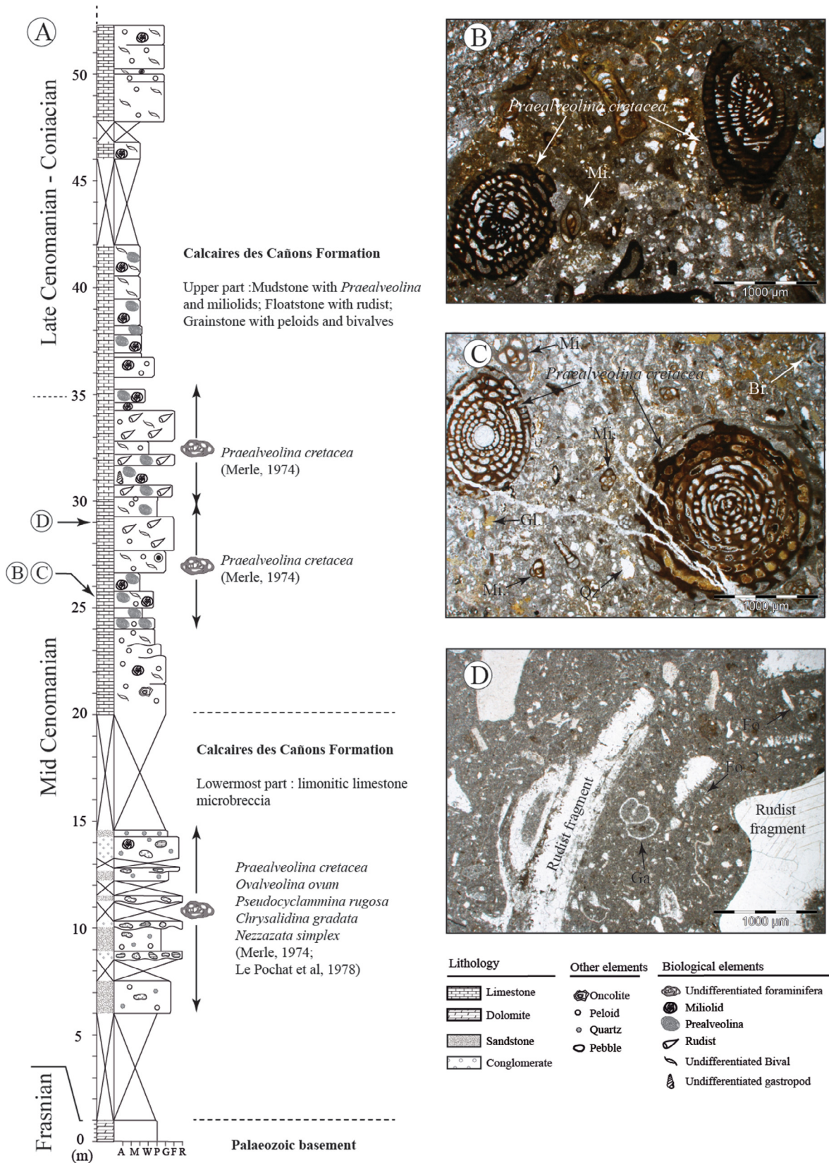
Fig 10. (A) Sedimentary log of the Calcaires des Cañons carbonate platform; (B, C) wackestone to packstone with Alveolina , miliolids (Mi.), bivalves (Bi.), quartz (Qz), and glauconite (Gl.); (D) wackestone rich in rudist fragments with well-preserved gastropods (Ga.) and foraminifers (Fo.) (from Saspiturry, 2019; Andrieu et al. , 2021).
