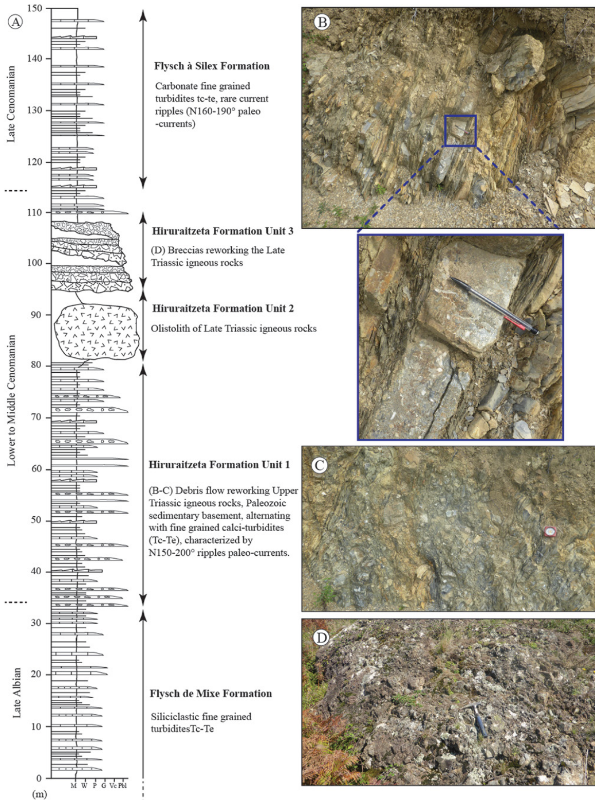
Fig. 9. Stratigraphy and lithology of the Hiruraitzeta Formation (A) Lithostratigraphic column at Hiruraitzeta (location in Fig. 3); (B) fine-grained calcareous turbidites with incomplete Bouma sequences, interfingering with out-of-sequence clast-supported polygenetic breccia with clasts of Paleozoic metasediments and Late Triassic igneous rocks; (C) meter-thick polygenetic breccia with clasts of Paleozoic metasediments and Late Triassic igneous rocks; (D) monogenetic clast-supported breccia of Late Triassic igneous rocks.
