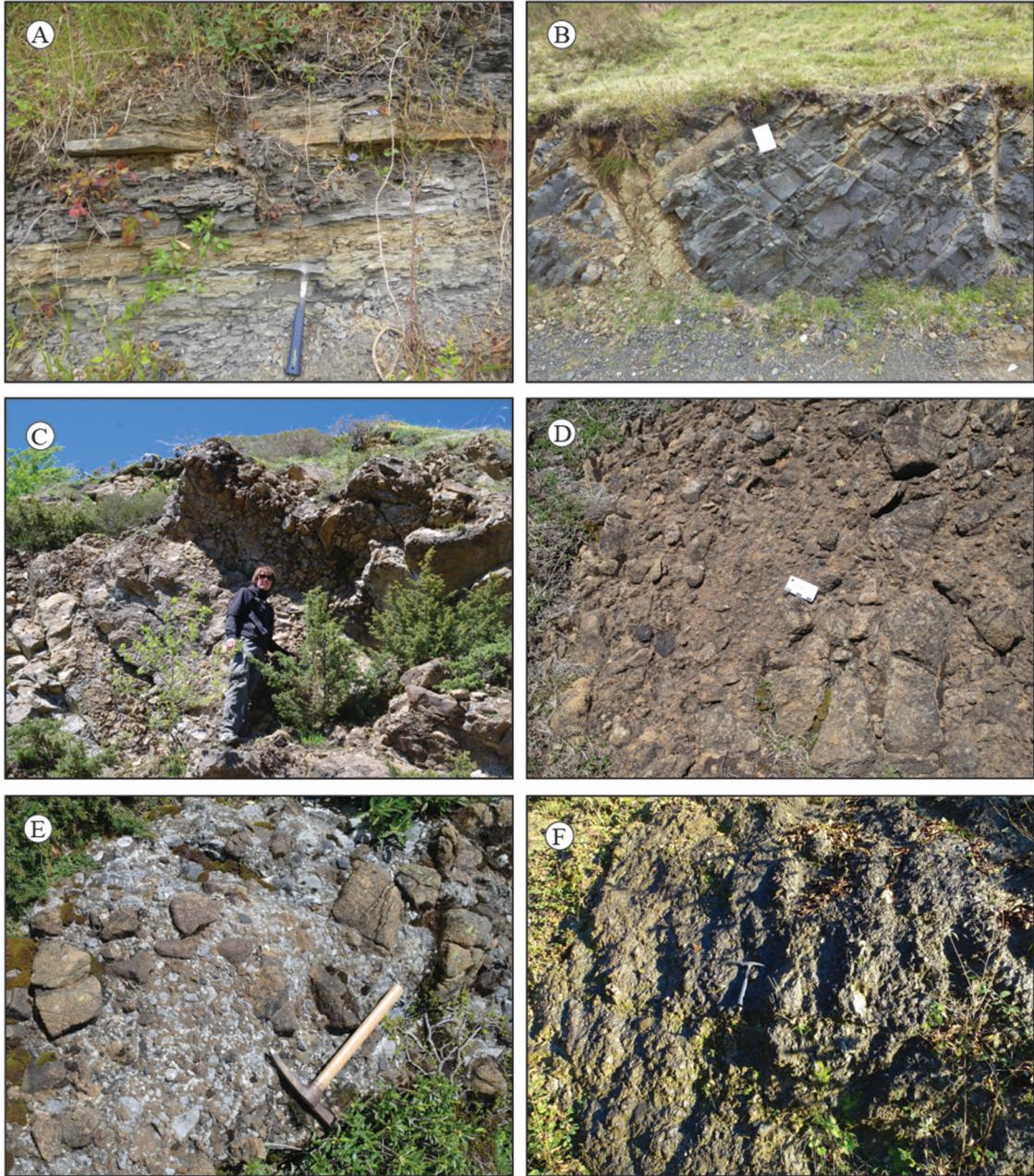
Fig. 6. Field photographs showing (A) micaceous silty marl of the Flysch de Mixe Formation with interbedded fine-grained Bouma-type turbidites; (B) serpentinized mantle rocks of the Urdach Member; (C) typical fresh lherzolite tectonic breccia in the Urdach area; (D) ophicalcite breccia made up of variably serpentinized lherzolite clasts in a calcitic matrix; (E) polymictic lherzolite-marble breccia made up of various types of high-temperature Mesozoic marble; (F) conglomerate of the Erretzu Member made up of centimeter-sized pebbles and subangular clasts.
