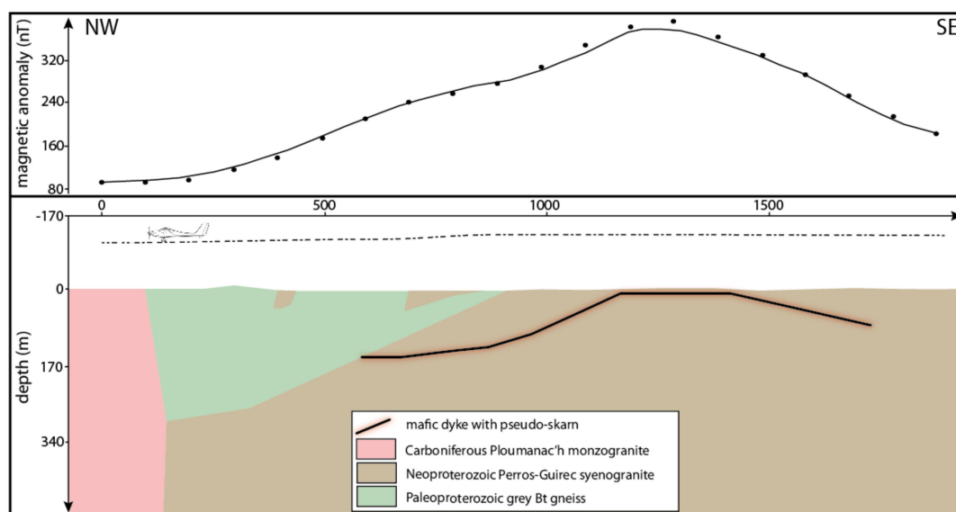
Figure 6. Regional magnetic modelling along the coast (profile location on Figure 4a). Upper window: measured regional magnetic anomaly (dots) compared to the computed magnetic model effect (line). Lower window: colors of modelled geological units are consistent with Figure 2. Taking into account a realistic “geological magnetic background”, a good fit of the regional magnetic anomaly can be achieved with a “ribbon-shaped” pseudo-skarn developed along a low-dipping mafic dyke (in black with red shadow—exaggerated in thickness). Vertical exaggeration is 1 for all displayed cross-sections.
