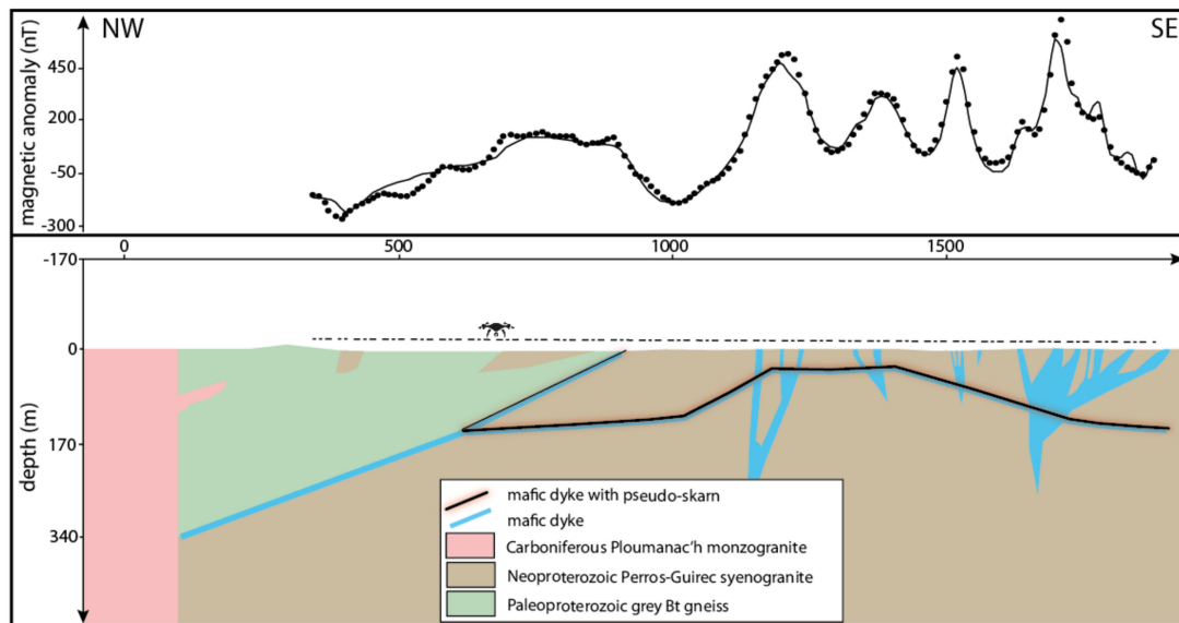
Figure 8. Local magnetic model along the coast: outcropping dykes and their actual measured magnetic susceptibility, as well as an ad hoc anastomosis at depth allow fitting the high resolution magnetic data. Upper window: UAV-borne measured magnetic anomaly (dots) compared to the computed magnetic model effect (line). Lower window: colors of modelled geological units are consistent with Figure 2.
