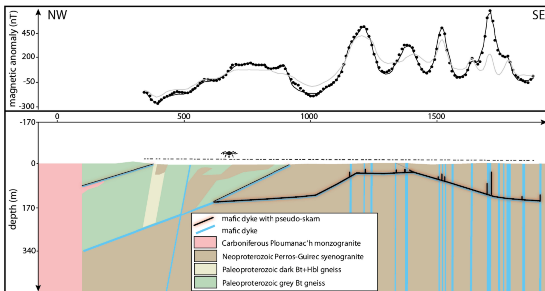
Figure 9. Final magnetic model along the coast. Upper window: UAV-borne measured magnetic anomaly (dots) compared to the computed magnetic model effect (line). Lower window: colors of modelled geological units are consistent with Figure 2. 1st and 3rd dolerite dyke generations are modelled as 2D subvertical sheets; their magnetic effect only cannot account for the entire magnetic signal (grey line in upper panel). For the final fit of the magnetic data (black line in upper panel), pseudo-skarn mineralization (in black with red shadow—exaggerated in size) was modelled channeled along some of the vertical dolerite dykes, in connection with the mineralized 2nd generation low-dipping mafic dyke.
