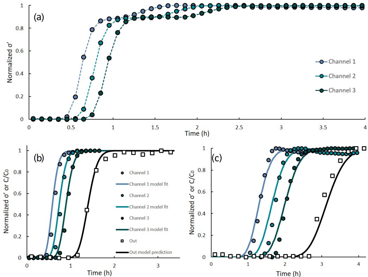
Figure 4. (a) Real conductivity at 1 Hz vs. time at three locations, (b) model fit to the \sigma'^- -based initial BT and model prediction for the non-reactive species at the outflow compared to their measured concentration and (c) model fit to the \sigma'^- -based secondary BT and model prediction for the reactive fraction of Ca^{2+} ions (calculated as outflow Ca^{2+} minus its “non-reactive fraction”) compared to its measured concentration.
