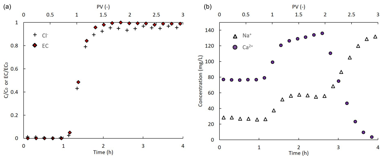
Figure 3. Outflow values vs. time (bottom horizontal axis) and pore volume (PV; upper horizontal axis) of (a) measured Cl^- and EC (‘+’ signs and red rhombi) and (b) Na^+ and Ca^{2+} ions (empty triangles and purple circles).
