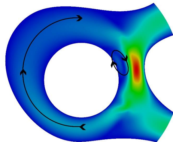
Figure B1 2D surface plot of velocity on the right side of the pore assembly: (a) Imbibition mechanism, and (b) Drainage mechanism; ( the arrows schematically show the rotation around the centroid, and colors show the velocity magnitude, blue color is low velocity zone and red color is high velocity zone).
