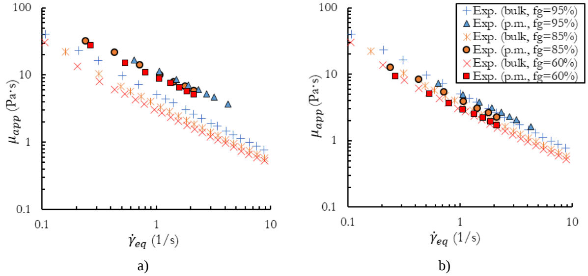
Fig. 9 Apparent viscosity vs shear rate a) experimental results b) fitted results with \alpha shift parameter
