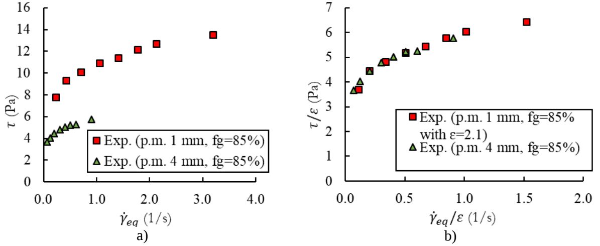
Fig. 15 Shear stress as a function of shear rate for foam quality of f_g = 85\% in 1 and 4 mm GB packings a) without expansion factor b) with \varepsilon=2.1 expansion factor for 1 mm GB packing
