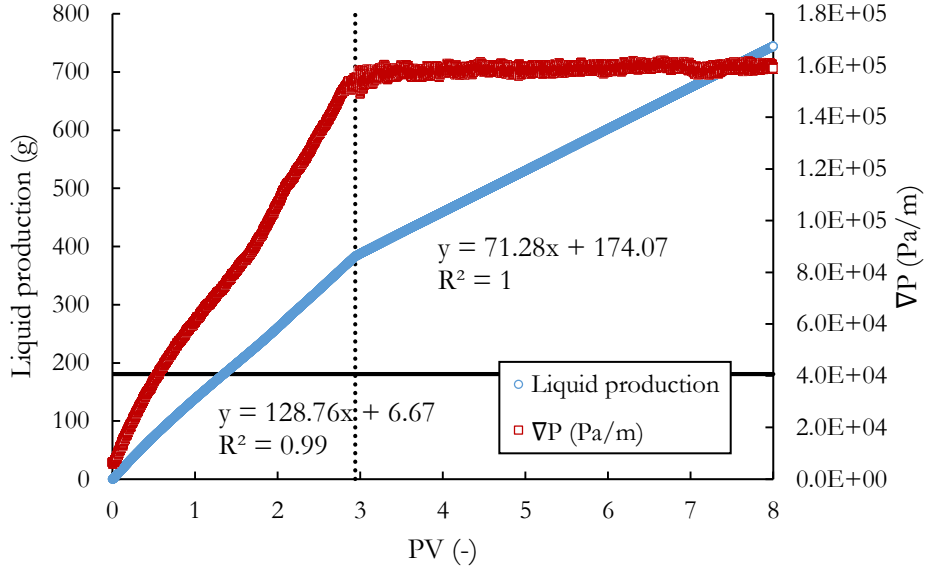
Fig. 13 Liquid mass of effluent as a function of PV for GB packing at Q_t=2 mL/min for f_g=60\%
