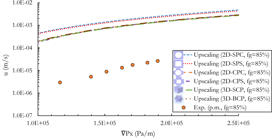
Fig. 11 The macroscopic pressure gradient vs. superficial velocity of foam flow in 2D SPC, SPS, CPC, CPS and 3D SCP, BCP unit cells ( f_g=85\% )
