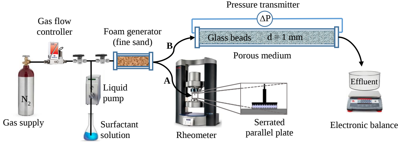
Fig. 1 Schematic of the experimental setups used to characterize the rheology of A) bulk foam and B) foam in porous media
