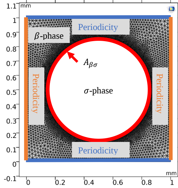
Fig. 4 The mesh and boundary conditions used to run the simulations
