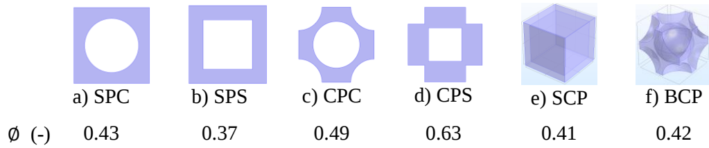
Fig. 3 2D and 3D periodic unit-cells for an array of parallel cylinders of circular (a, c), square (b, d) cross-sections, (e, f) simple cubic and cubic body-centered packings
