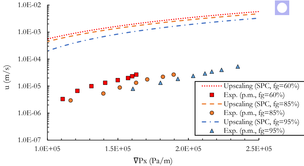
Fig. 10 Evaluation of the superficial velocity as a function of the macroscopic pressure gradient in 2D periodic SPC geometry, for different foam qualities ( f_g=60, 85 and 95\% )
