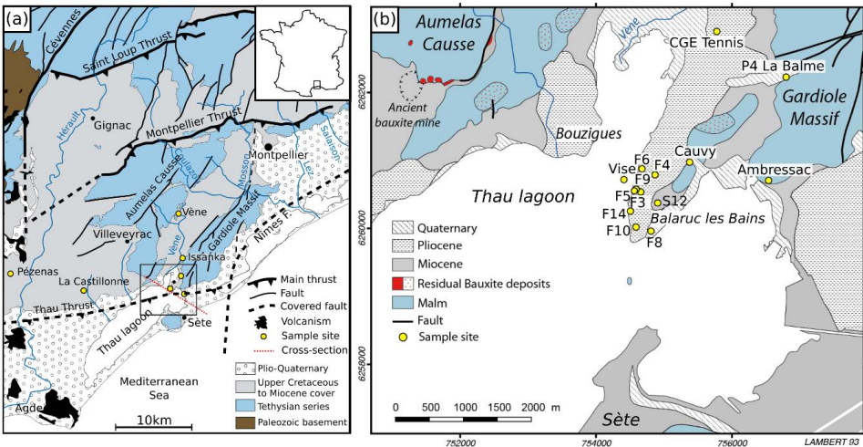
138 139 Figure 1 (a) Simplified geological map showing the main structures of the Montpellier region. The box locates the 140 Balaruc-les-bains study area, between the Montpellier thrust and the Nîmes Fault. (b) Detailed geological map 141 of the eastern Thau lagoon. Sample sites indicated by the yellow dots in both maps correspond to the locations of 142 the thermal wells, karst springs, and other piezometric drilling sites. The location of the ancient bauxite mine 143 (Cambelliès) is indicated by the dashed oval in the northwest of the study area.
