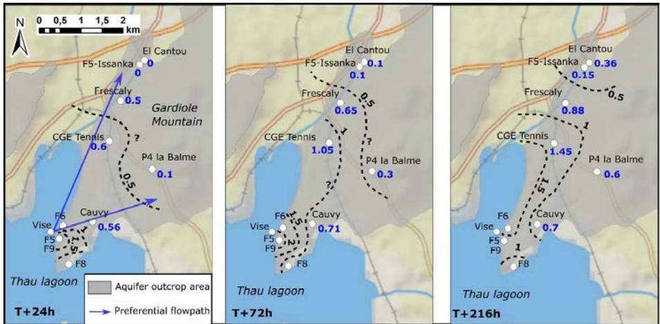
352 Figure 4 Spatial propagation of the hydraulic perturbation (hydraulic head increase in m) across the Balaruc-les- 353 Bains peninsula during the 2014 inversac event at three times after initiation: T+24 h, T+72 h, and T+216 h.
