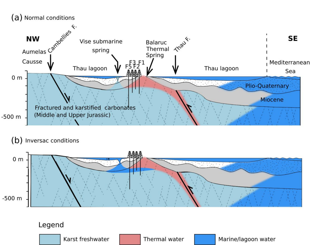
287 Figure 2: Conceptual cross-section oriented NW-SE passing through thermal wells of the Balaruc peninsula, and 288 showing groundwater flows of the karst hydrosystem under (a) normal conditions and (b) inversac conditions. 289 Location of the cross-section is indicated in Figure 1a.
