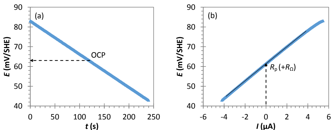
Figure 12. Example of an LPR measurement in the cathodic direction from +20\text{ mV} to -20\text{ mV} vs. OCP. (a) Evolution of the potential with time applying a potential sweep of 10\text{ mV min}^{-1} , (b) Evolution of the potential with a current during the potential sweep, allowing the determination of R_p .
