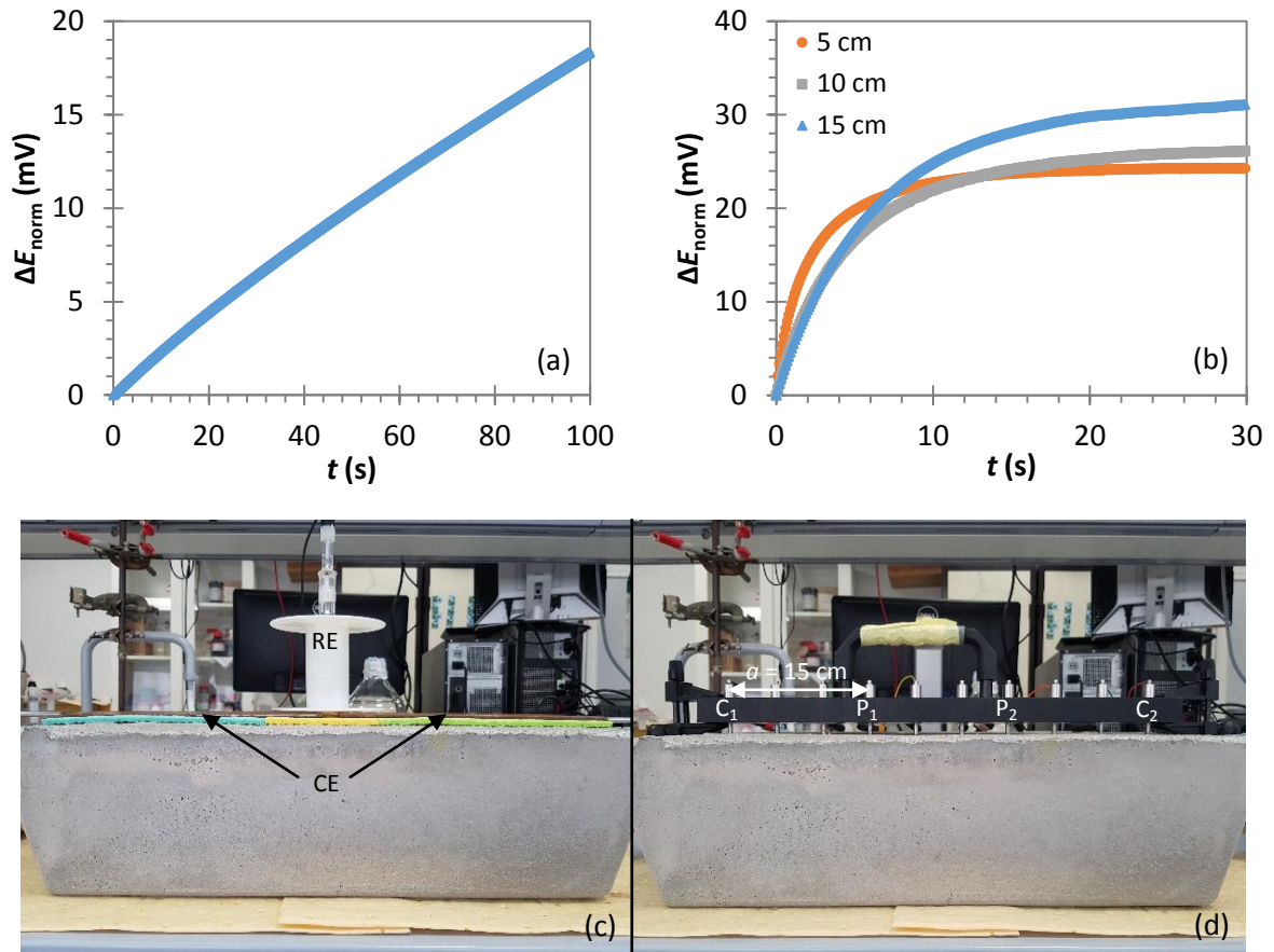
Figure 17. GP measurements using (a) three-electrode and (b) four-electrode configurations on a passive rebar. Experiments were done on a CEM I 52.5R (Lafarge) mortar sample ( 55 \times 34 \times 13 \text{ cm}^3 , w/c=0.4 ) with one ribbed carbon steel rebar (60 cm, \Phi=12 \text{ mm} , cover depth 3.3 cm), at constant relative humidity (dry conditions, \approx 30\text{--}40\% RH) and temperature ( 23^\circ\text{C} ). In the three-electrode configurations (c), measurements were conducted with a mercury/mercurous sulphate reference electrode located at the centre of the sample, and a stainless-steel counter electrode ( 55 \times 10 \text{ cm} ) placed on moist sponges on the sample surface directly above the rebar. In the four-electrode configuration (d), stainless-steel or brass electrodes ( \Phi_i=3 \text{ mm} , \Phi_e=5 \text{ mm} ) were used in Wenner configuration, centred directly above and parallel to the rebar. The electrolytic contact was made with moist sponges placed inside the probes. Electrode spacing a was 5, 10 or 15 cm. A potentiostat-galvanostat (PMC-2000, Princeton Applied Research) was used for galvanostatic pulse measurements. The impressed current was 10 \mu\text{A} between rebar and counter electrode in the three-electrode configuration, while it was 200 \mu\text{A} between C_1 and C_2 in the four-electrode configuration. The results indicate that a quasi-steady-state is not reached after 100 s in the three-point configuration, while it is almost reached after 30 s in the four-point configuration.
