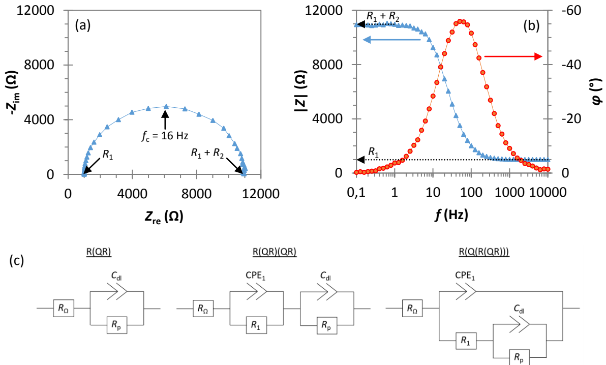
1012 Figure 15. Example of (a) Nyquist plot and (b) Bode plot obtained at 10 mV RMS between 10^4 and 10^{-1} Hz with 1013 10 points per decade using a dummy cell with parameters R_1=1000 \Omega , R_2=10000 \Omega and C=1 \mu F . (c) Examples of 1014 electrical equivalent circuits for fitting the experimental results in the case of steel corrosion in concrete, from 1015 left to right: R(QR) , R(QR)(QR) and R(Q(R(QR))) . In addition to the resistance of the electrolyte, the polarization 1016 resistance and the double layer capacitance, the additional parameters can be attributed to the passive film.
