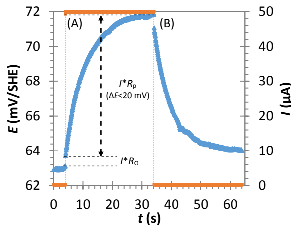
Figure 13. Example of GP measurement in the anodic direction showing the injection of 50 \mu A during 30 s and the evolution of \Delta E with time during (A) the charge (current applied) and (B) the discharge (no current applied).
