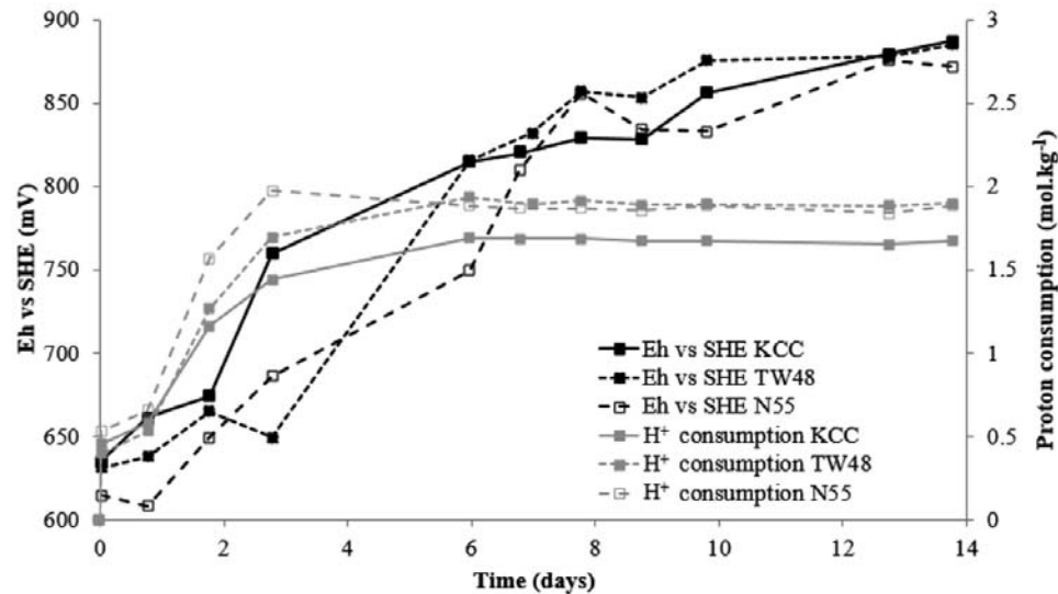
Fig. 3. Redox potential and protons consumption over time for the experiments with the three different consortia at 42, 48 and 55 °C.
