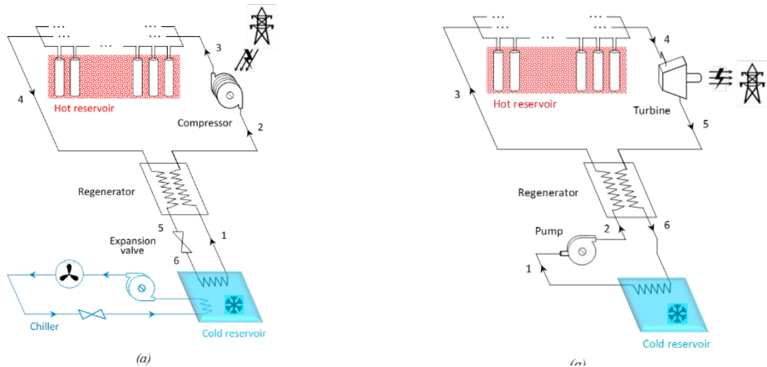
Figure 1: a) Charging process, b) Discharging process
