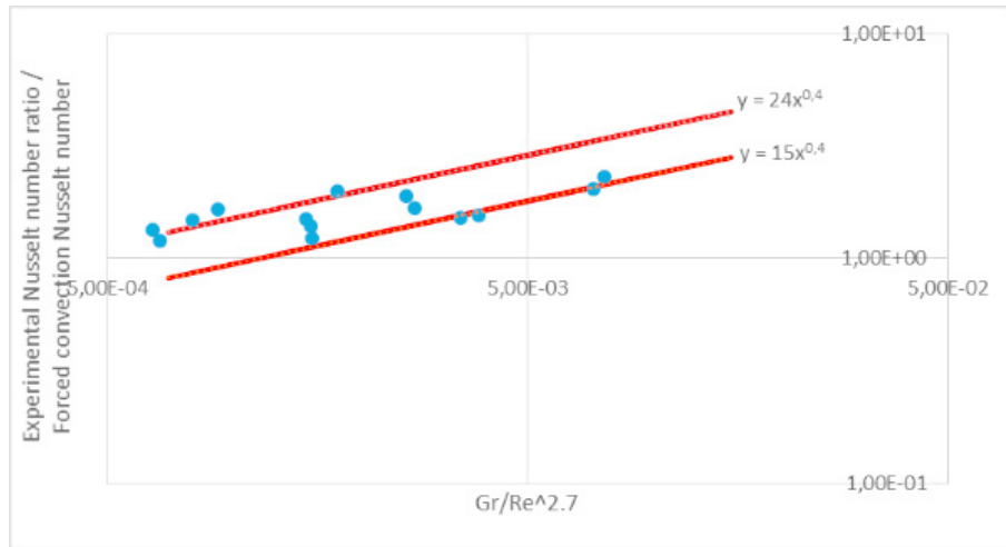
Figure 9. Nusselt number ratios vs Gr/Re^{2.7}
