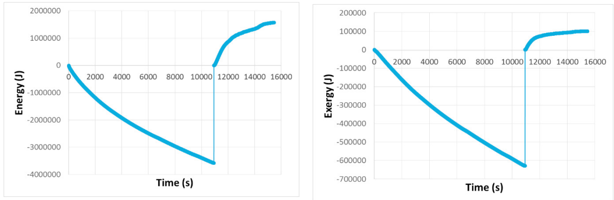
Figure 5. Evolution of cumulated energy (left) and exergy (right)
