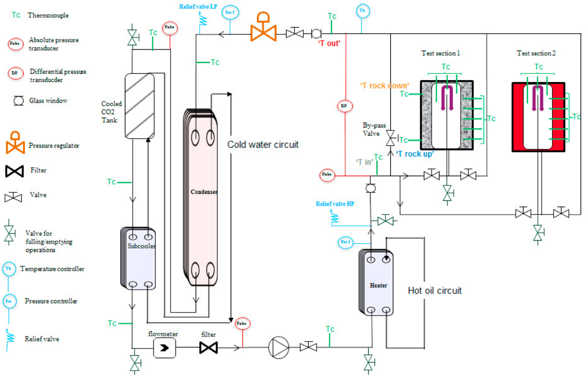
Figure 2. Schematic draw of CO 2 loop
