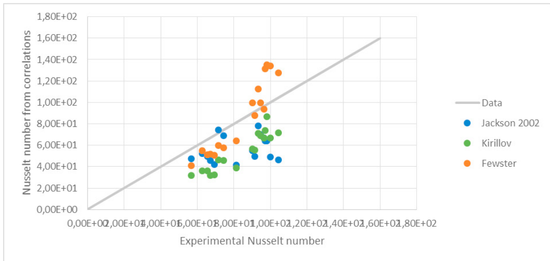
Figure 8. Nusselt number from different correlations vs experimental Nusselt number
