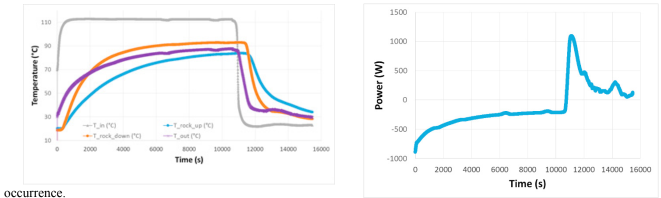
Figure 4. Evolution of temperature (left) and heat rate (right). Locations of thermocouples are mentioned in Fig. 2.
