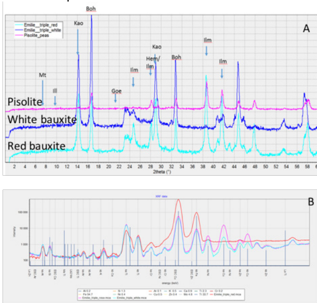
Figure 7. A. Diffractograms of red (light blue) and white (dark blue) bauxite and pisolite (red). B. XRF spectra of the same sample.
