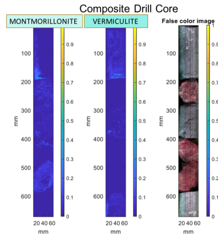
Figure 5. Artificial composite drill core of the major facies of the bauxite mine, showing the major mineralogy mapped by SOLSA software using SWIR hyperspectral data. Marls is sonic drilled.
