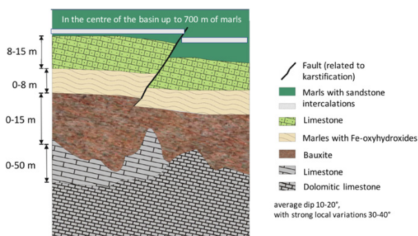
Figure 1. Schematic lithological profile at the bauxite deposit (Villeveyrac, France) (modified from Giroud et al. 2009).
