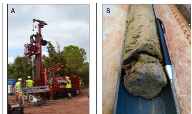
Figure 2. A. SOLSA Drill at the bauxite mine (SODICAPEI), B. variegated marls.
