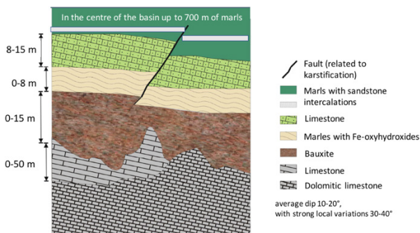
Figure 1. Schematic lithological profile at the bauxite deposit (Villeveyrac, France) (modified from Giroud et al. 2009).
