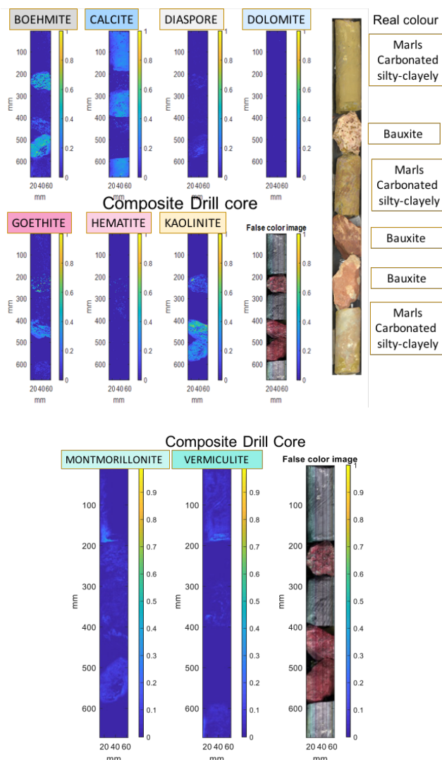
Figure 5. Artificial composite drill core of the major facies of the bauxite mine, showing the major mineralogy mapped by SOLSA software using SWIR hyperspectral data. Marls is sonic drilled.
