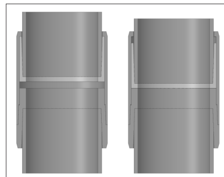
Fig. 2 Concept drawing revealing the main principles of the flexible coupling. On the left is the coupling shown in open mode, on the right in closed mode. (Patent application no. 050129 – Thorbjörnsson 2015)
