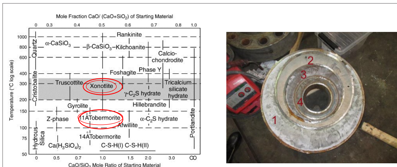
Fig. 1 Phases that occur in cement depending on Ca/Si ratio and temperature (left, from Meller et al. after Taylor [1, 2] ; red-rimmed minerals were found in IDDP-1 cement) and picture of top view of the retrieved casings at the top of the IDDP-1 well (right). (1–4: cement layers)
