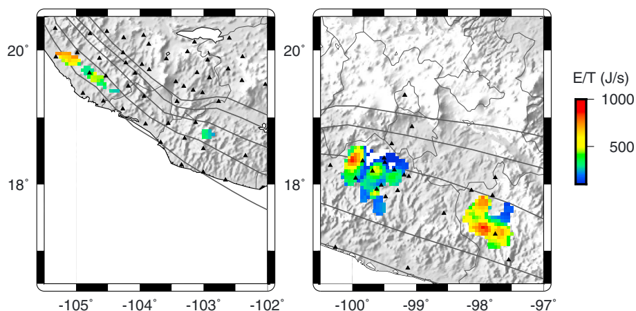
Figure 6. Spatial distribution of tremor energy rates defined as the median of the size-frequency statistic (Yabe & Ide, 2014). A grid of 0.05^\circ is defined, and the energy rate is calculated for points with more than 50 tremors within a 10 km radius.
