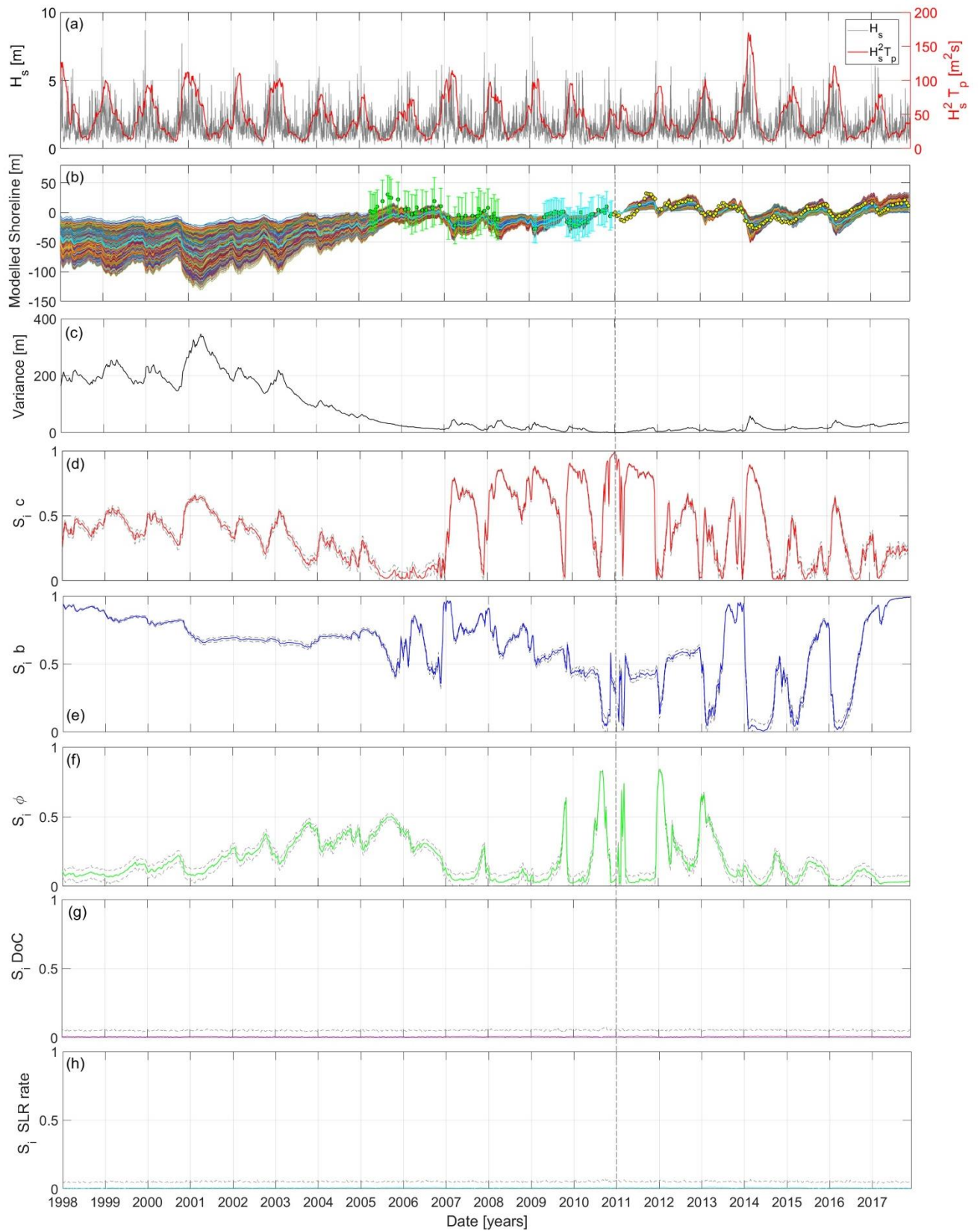
Figure 6 (a) Simulated offshore wave conditions synthesized in the average value H_{s0}^2/T_p ; (b) Envelope of 3000 simulated shoreline over the period 1998-2018 (coloured lines), and observed average shoreline positions between 2005 and 2017 (green before 2011 and yellow dots after 2011) with bars indicating the estimated maximum possible
