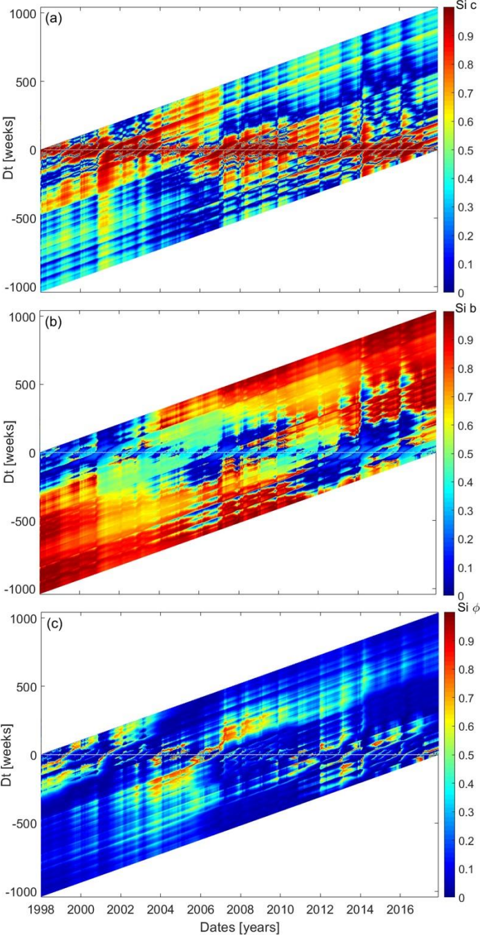
Figure 7 1 st order Sobol' index time series calculated for (a) c ; (b) b ; and (c) \phi parameters
