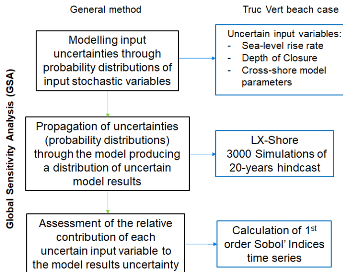
Figure 4 Schematic representation of the method developed herein
