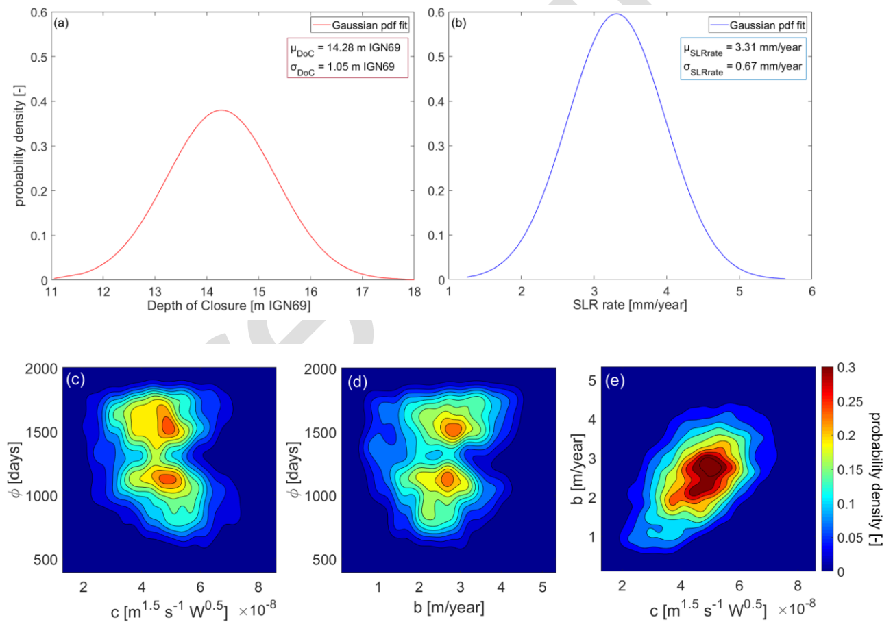
Figure 5 Probability density functions of: (a) DoC; (b) SLR rate; (c), (d) and (e) (c, \phi) , (b, \phi) and (c, b) cross-shore module parameters respectively
