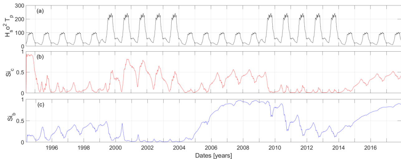
Figure 10 Idealized alternate low-energy and high-energy winters every 4 years. (a) Simulated seasonal wave conditions; (b) and (c) Sobol' indices of the free parameters c and b respectively
