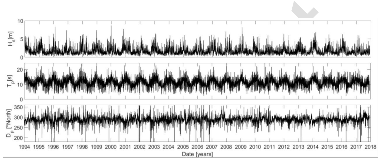
Figure 2 NORGAS-UG wave hindcast time series from 1994 to 2018 at (44°39'9" N; -1°26'48" W) offshore of Truc Vert beach (see Figure 1a): (a) significant wave height; (b) peak wave period; and (c) peak wave direction expressed in Nautical convention
