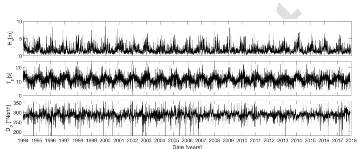
Figure 2 NORGAS-UG wave hindcast time series from 1994 to 2018 at (44°39'9" N; -1°26'48" W) offshore of Truc Vert beach (see Figure 1a): (a) significant wave height; (b) peak wave period; and (c) peak wave direction expressed in Nautical convention
