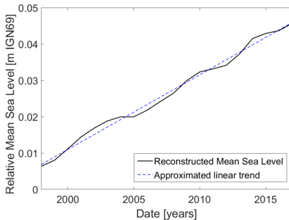
Figure 3 Relative Mean Sea Level time series relative to Cap-Ferret land elevation (m NGF IGN69), with linear approximations over 1998-2018
