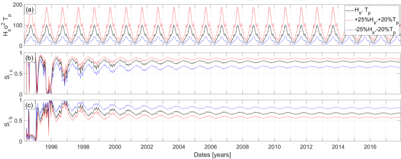
Figure 9 Idealized seasonal wave climate, with increased (red curves) and decreased (blue curves) intensity. (a) Simulated seasonal wave conditions; (b) and (c) Sobol' indices of the free parameters c and b respectively
