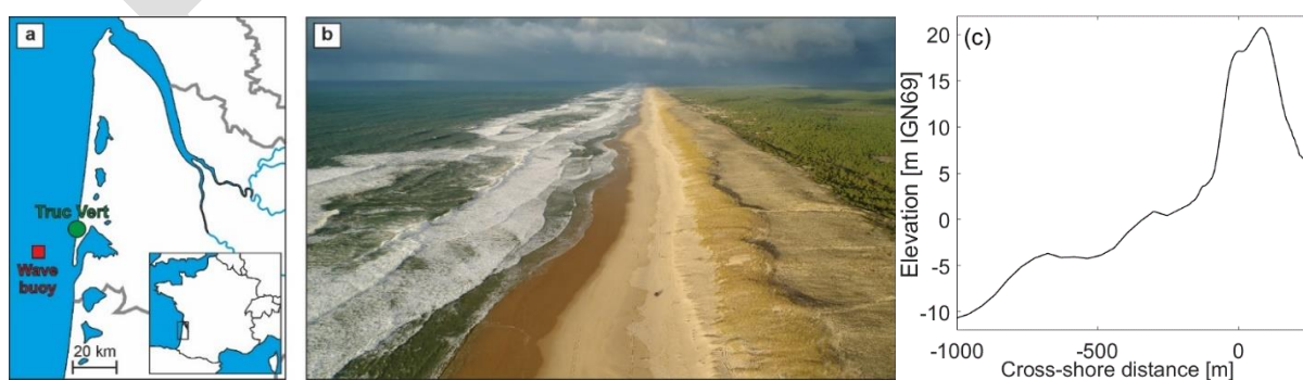
Figure 1 (a) Location of Truc Vert beach (green) and of the wave hindcast grid point co-located with Candhis in situ wave buoy (red); (b) picture of Truc Vert beach landscape (Photo from V. Marieu); and (c) alongshore-averaged
