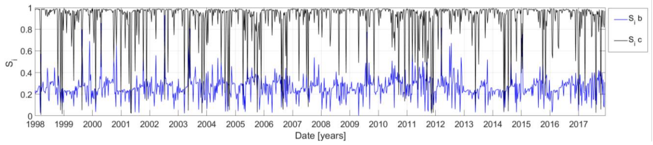
Figure 8 Progressive ( Dt = 1 week) 1 st order Sobol' index time series for c and b
