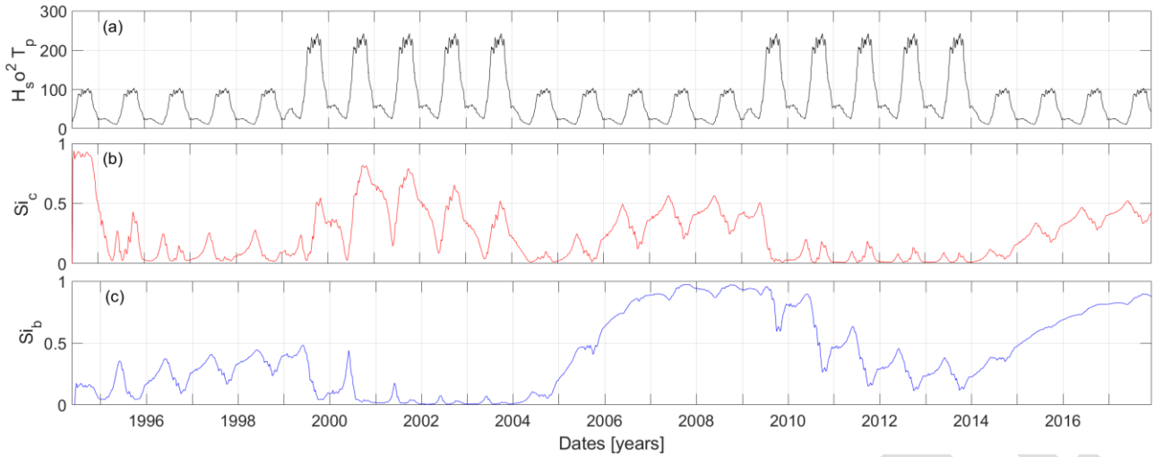
Figure 10 Idealized alternate low-energy and high-energy winters every 4 years. (a) Simulated seasonal wave conditions; (b) and (c) Sobol' indices of the free parameters c and b respectively
