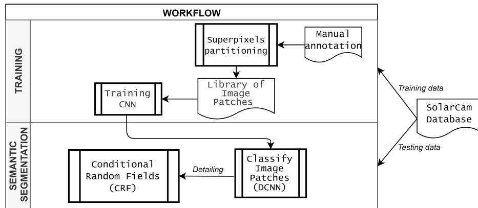
Figure 2. Workflow of the methodology: training phase useful for building the models by means of convolutional neural network (CNN) transfer learning mechanism, by using superpixel-based patches and the semantic segmentation phase, whose results are used for testing the pixel-scale classification accuracy. DCNN: deep CNN.
