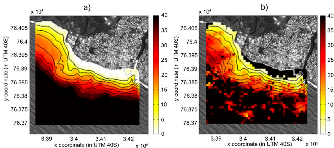
Figure 10. The bathymetry: (a) measured; and (b) estimated by the CWB (in m) method on the area of Saint Pierre on Reunion Island. The isobaths represented in black range from 0 to 50 m depth with a step of 5 m (from [98]).
