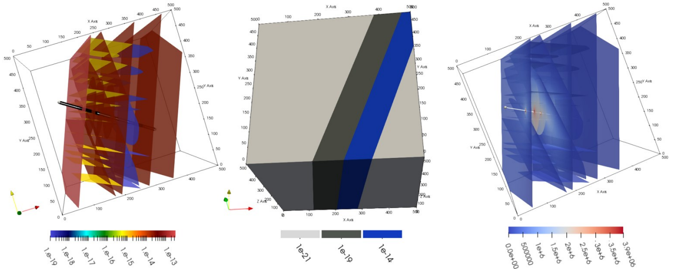
Figure 4. Initial model (reference); Left: Permeability of fractures (m 2 ); Middle: Permeability of subdomains; Distribution of the differential of pressure (Pa) between initial state and after 12 h of injection
