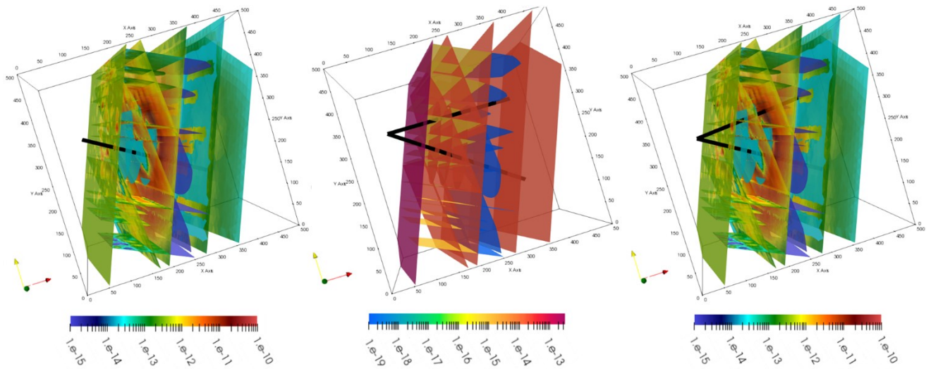
Figure 5. Permeability distribution for each model and well architecture. Left: Permeability resulting from hydraulic stimulation. Middle: Well architecture (two-legs). Right: Combined method: Hydraulic stimulation and well architecture are both deployed.
