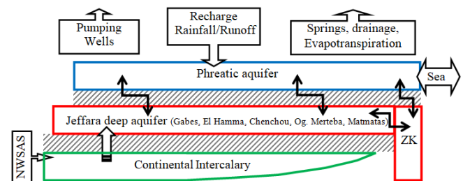
Fig. 1 Conceptual model of Gabes Jeffara aquifers
