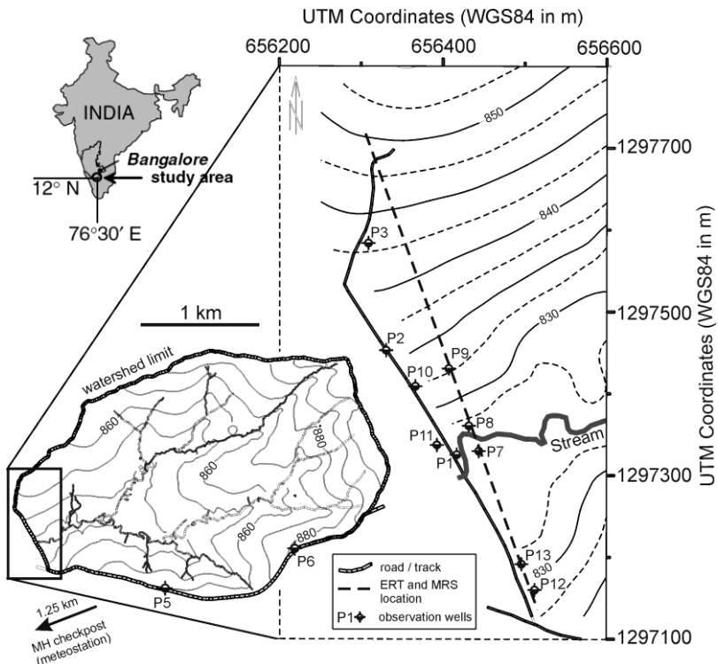
Fig. 2.2-1 - Location map of the experimental site at the outlet of the Mule Hole watershed (modified from Desclouetres et al., 2008). Collapsed observation well P4 is not represented (elevation in MASL).
