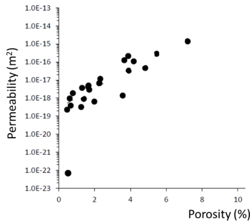
Figure 2: Permeability of Ringelbach’s core samples as a function of the porosity of the samples (Belghoul, 2007).
