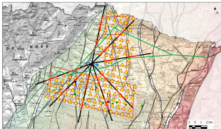
Figure 9: Planned 3D CSEM survey (receivers as yellow triangles, transmitter as a blue arrow) over the Sultz-sous-Forêts and Rittershoffen geothermal plants.
