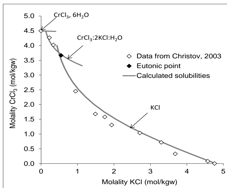
Fig. 1(a,b). Experimental (symbols) and predicted (lines) \text{KCl(s)} , \text{AlCl}_3\cdot 6\text{H}_2\text{O(s)} , \text{CrCl}_3\cdot 6\text{H}_2\text{O(s)} and 2\text{KCl}\cdot\text{CrCl}_3\cdot \text{H}_2\text{O (s)} solubilities in \text{KCl-AlCl}_3\text{-H}_2\text{O} (a), and \text{KCl-CrCl}_3\text{-H}_2\text{O} (b) systems at 25^\circ\text{C} . The solid
