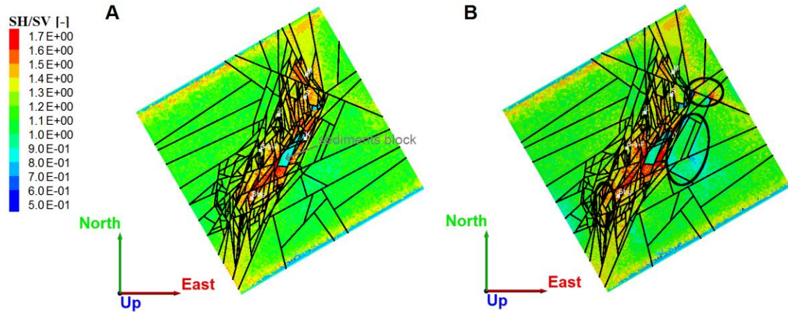
Figure 2. Ratio of maximum horizontal stress over vertical stress. A. Model 1. A grey arrow indicates the block of sediments. B. Model 2. Black ellipses indicate areas presenting variations from model 1. Faults are in black. Main cities plotted in Figure 1 are plotted here in blue with one letter for label.
